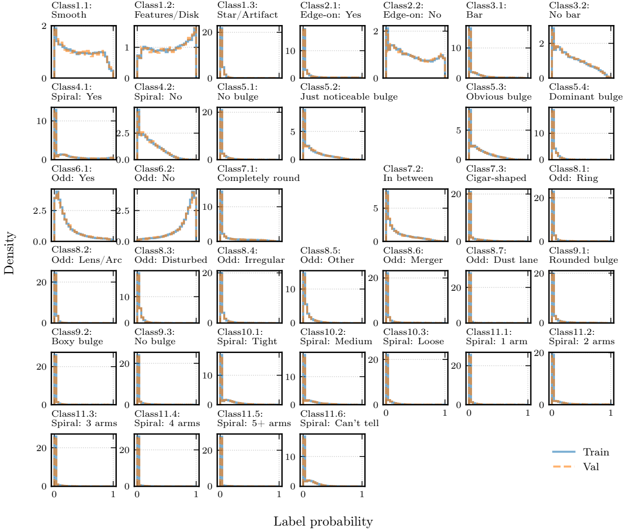
Fig. 9.— Per-label normalized histograms of the 80/20 train (blue) and validation (orange) split (seed 42). The two distributions overlap to within visible per-bin counting noise on every one of the 37 labels, confirming that the random split has not introduced any systematic label-prevalence drift between training and validation.
