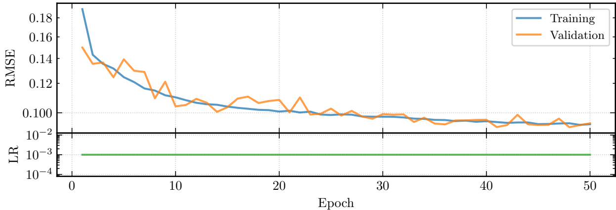
Custom CNN + Augmentation
