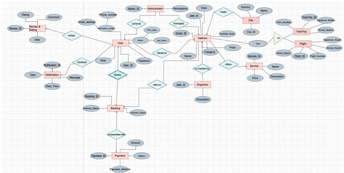
Figure 1: ER Diagram of Trips and Events Management System.
