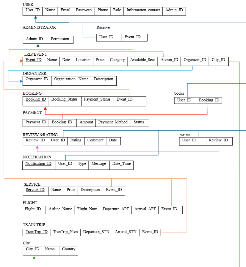
Figure 2: Mapping ER Shema of Trips and Events Management System.
