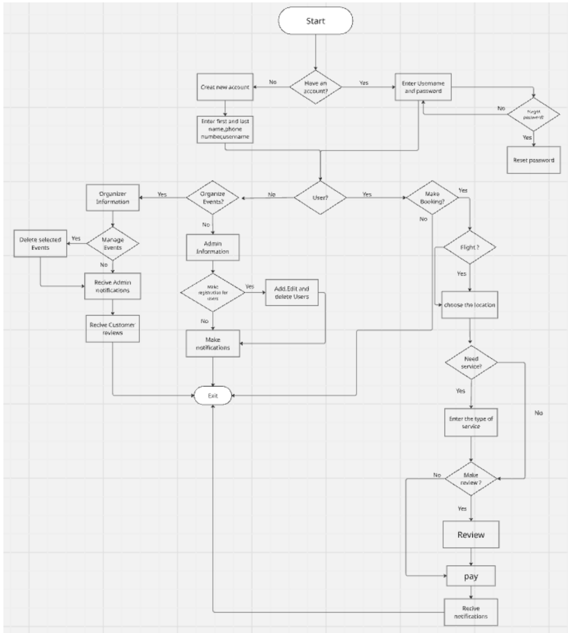
Figure 16: Flowchart Showing the Application Process.
