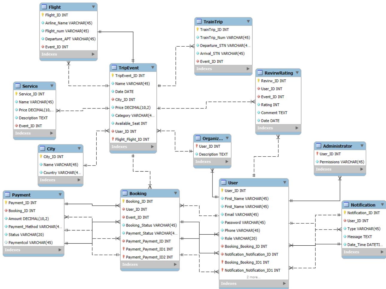
Figure 3: Explanation of The Relationships of Trips and Events Management System.
