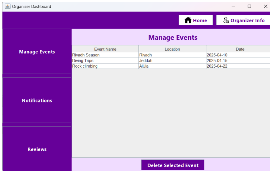
Figure 35: Organizer event management screen.
