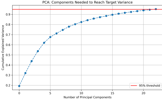
Figure 4: Cumulative explained variance plot for PCA. Retaining \sim 23 components preserves 95% of original dataset variance.
