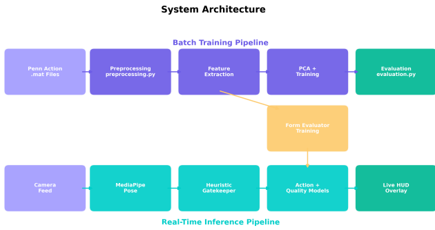
Figure 1: System Architecture Diagram detailing the data flow from raw RGB frames through MediaPipe spatial extraction, gatekeeping, decoupled asynchronous buffers, and the dual-stage classification and quality scoring modules.
