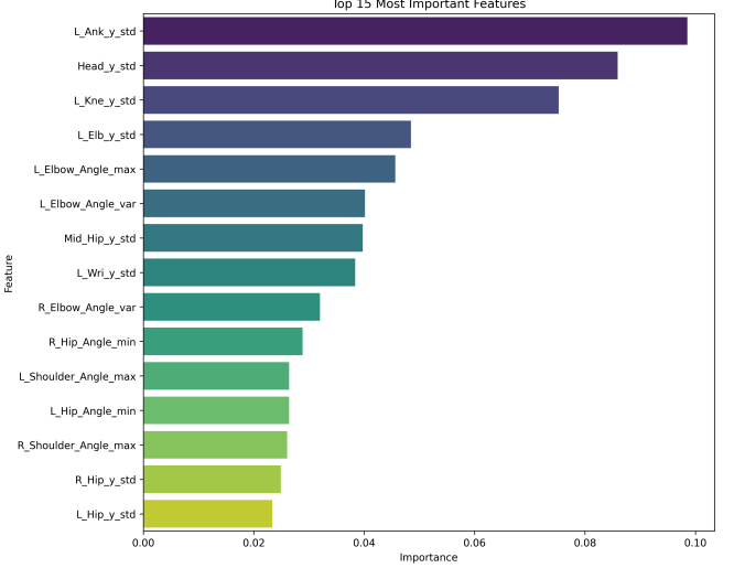
Figure 3: Top kinematic features as weighted by the Random Forest classifier. Statistical properties representing spatial variance (e.g., standard deviation of coordinates) proved highly discriminative for mapping execution patterns.
