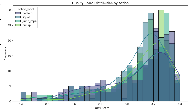
Figure 6: Distribution of Isolation Forest quality scores across different activities, reflecting the natural variability in unconstrained exercise execution.
