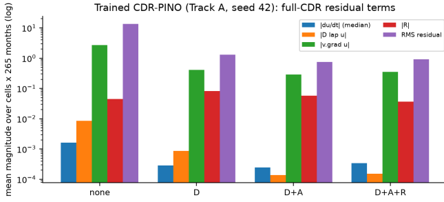
Fig. 6. Mean magnitudes of the rate of change, of each right-side term and of the residual for trained track A checkpoints (log scale).
