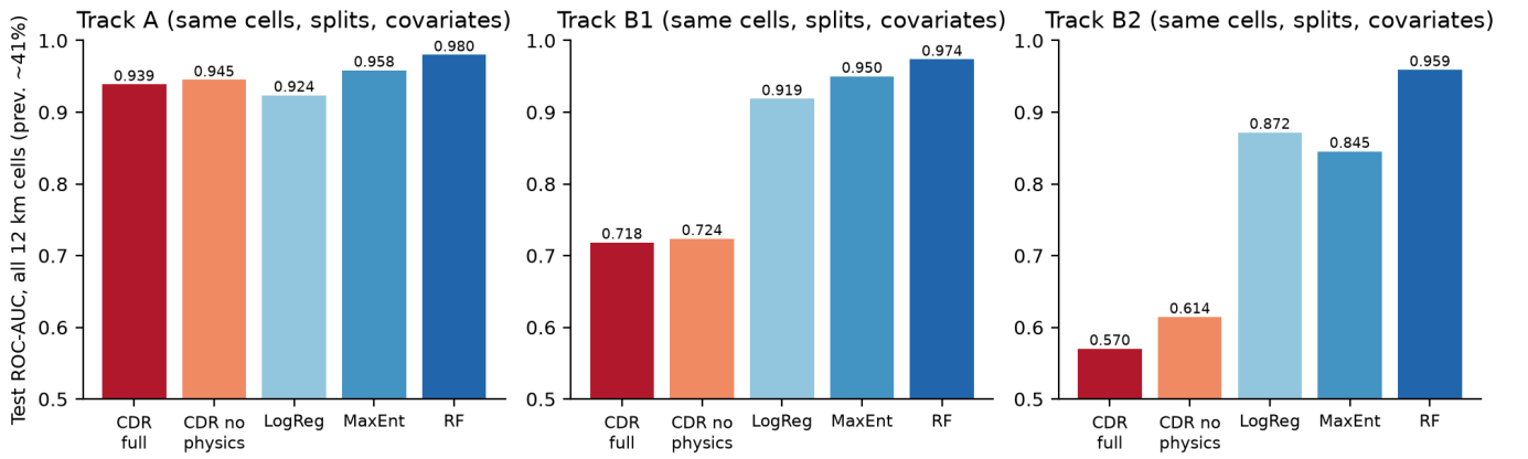
Fig. 4. Test ROC-AUC of the operator and of classical learners fitted on the same 12 km cells, partitions and seven covariates, for random cells (A), spatial blocks (B1) and held-out regions (B2).
