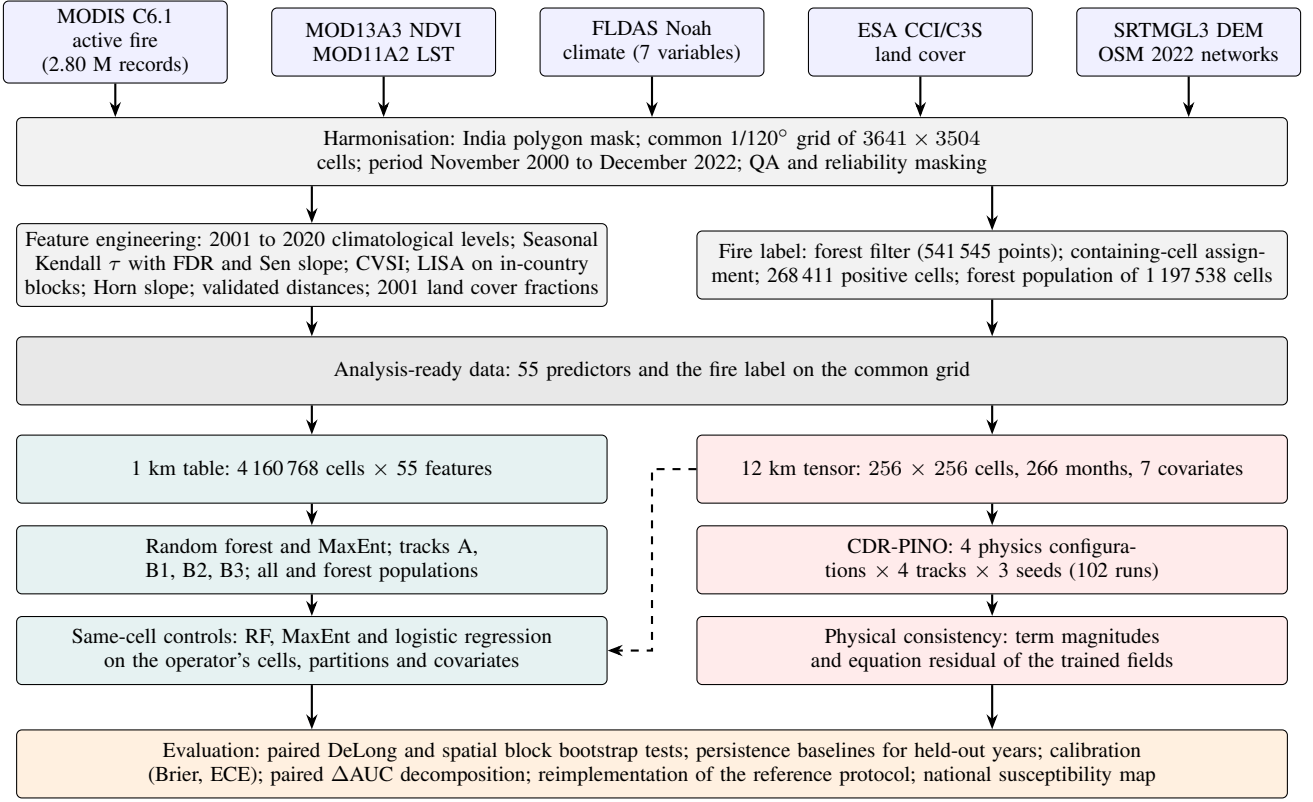
Fig. 1. Workflow of the study. Blue boxes are raw data products, grey boxes are shared preprocessing, green boxes form the classical branch at 1 km, red boxes form the operator branch at 12 km and the orange box is the common evaluation stage. The dashed arrow indicates that the same-cell controls are fitted on the operator's own tensor, cells and partitions.
