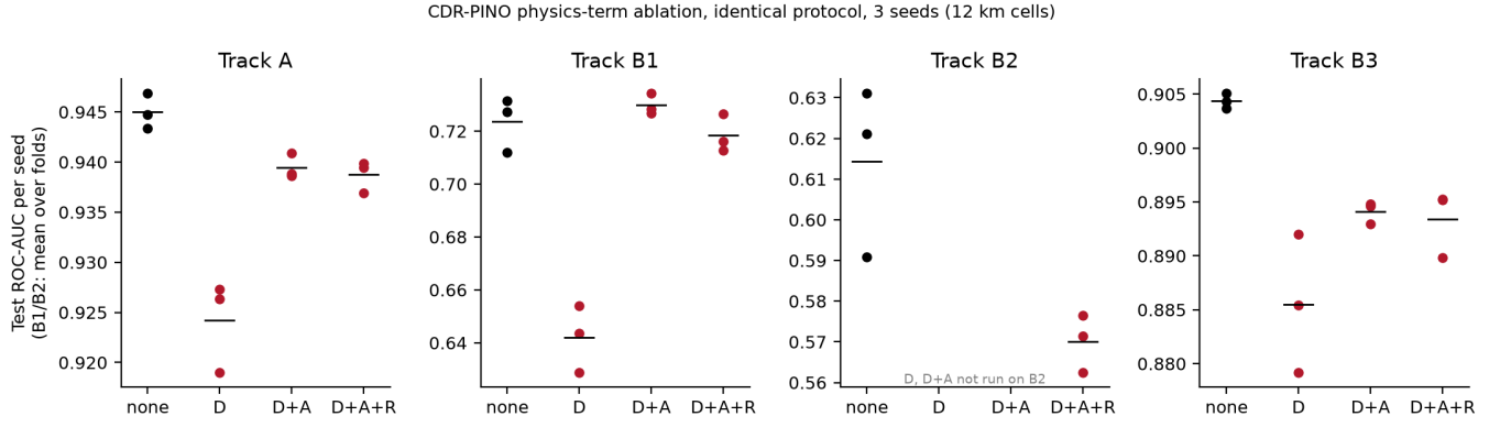
Fig. 3. Physics term ablation of the operator under an identical protocol. Dots are seeds (for B1 and B2, the mean over folds), horizontal lines are means. D, A and R denote diffusion, advection and reaction. Diffusion and diffusion with advection were not trained on track B2.
