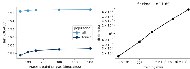
Fig. 10. MaxEnt test ROC-AUC and fitting time as a function of the number of training rows (50 000 to 500 000).
