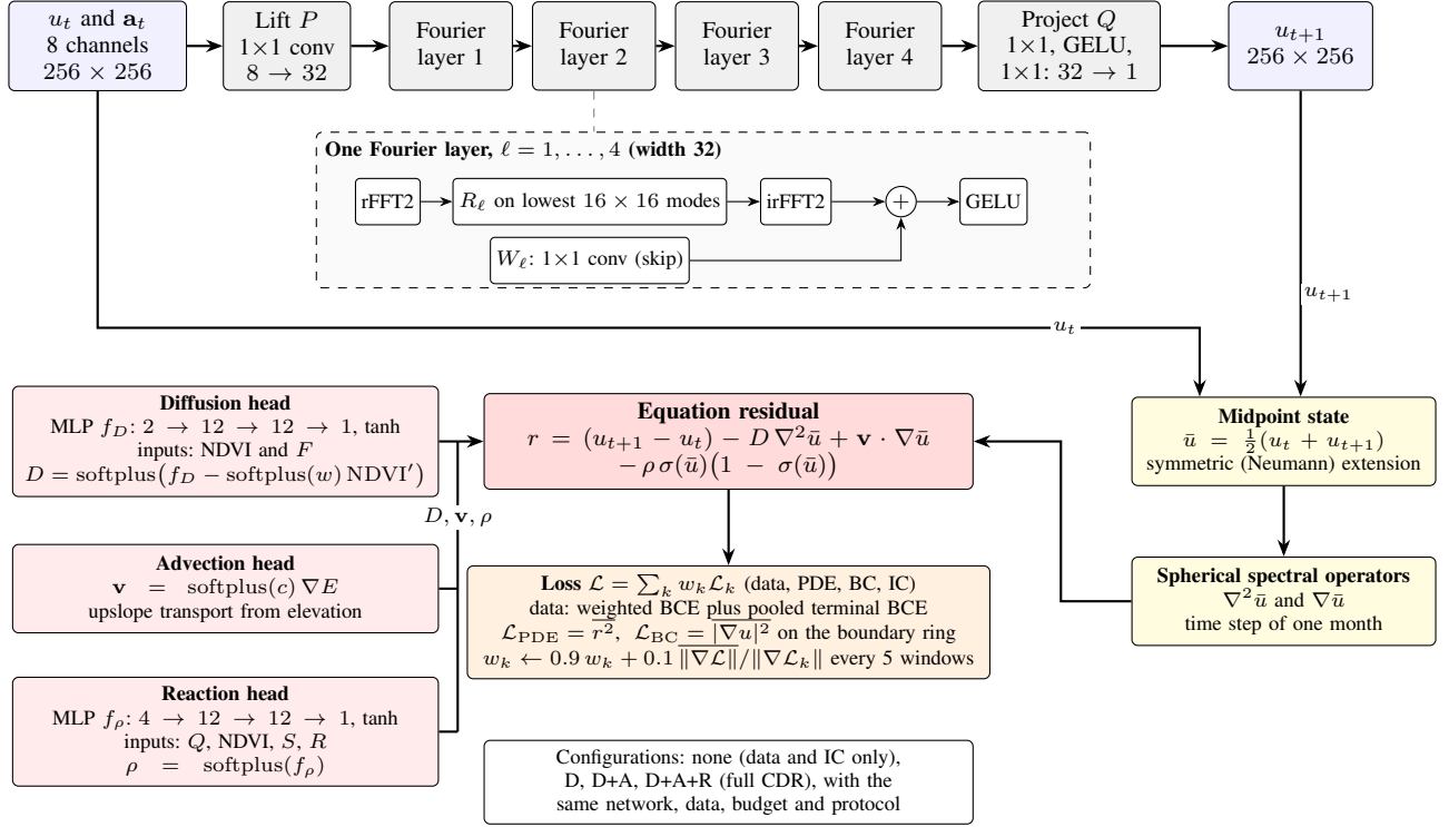
Fig. 2. Architecture of the CDR physics-informed neural operator. Top: the Fourier neural operator maps the state u_t and seven covariates of month t to u_{t+1} , with the structure of one Fourier layer shown in the inset. Bottom: three coefficient heads produce D , \mathbf{v} and \rho , spherical spectral derivatives are evaluated on the midpoint state, and the equation residual enters the loss together with the data, boundary and initial terms under adaptive weights. The initial condition u_0 = 0 is imposed exactly, so \mathcal{L}_{\text{IC}} is identically zero. The four physics configurations differ only in which terms enter the residual.
