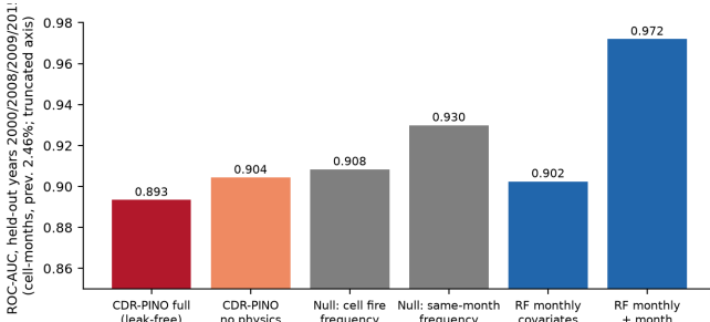
Fig. 5. Held-out years (2000, 2008, 2009, 2015) scored per cell and month. The operator is compared with two covariate-free baselines and with random forests on monthly covariates.
