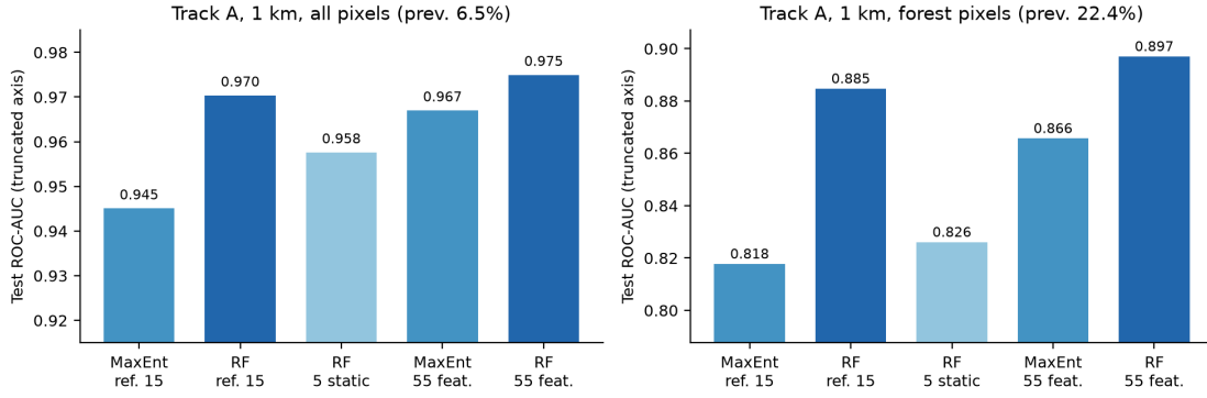
Fig. 7. Track A test ROC-AUC at 1 km for MaxEnt and random forest with the reference fifteen predictors (ref. 15), the operator's five static covariates (5 static) and the full 55 features (55 feat.), over all cells (left, prevalence 6.5%) and forest cells (right, prevalence 22.4%). The vertical axes are truncated.
