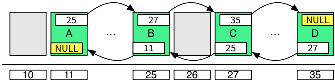
Figure 4.4 A double Linked List in the computer's memory.
