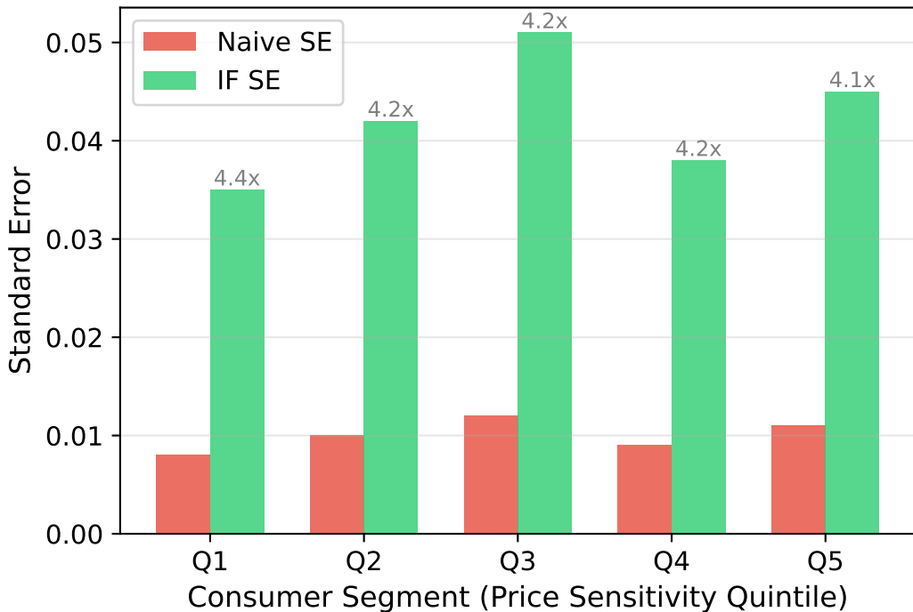
Naive vs IF Standard Errors by Segment
