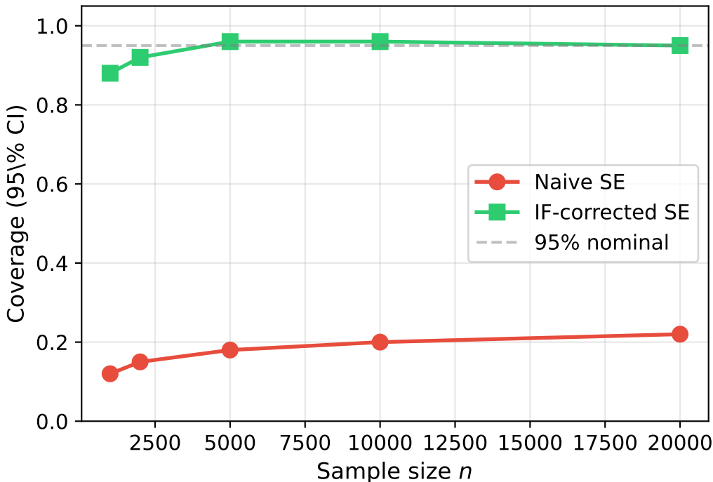
Naive vs IF Coverage (Binary Logit)
