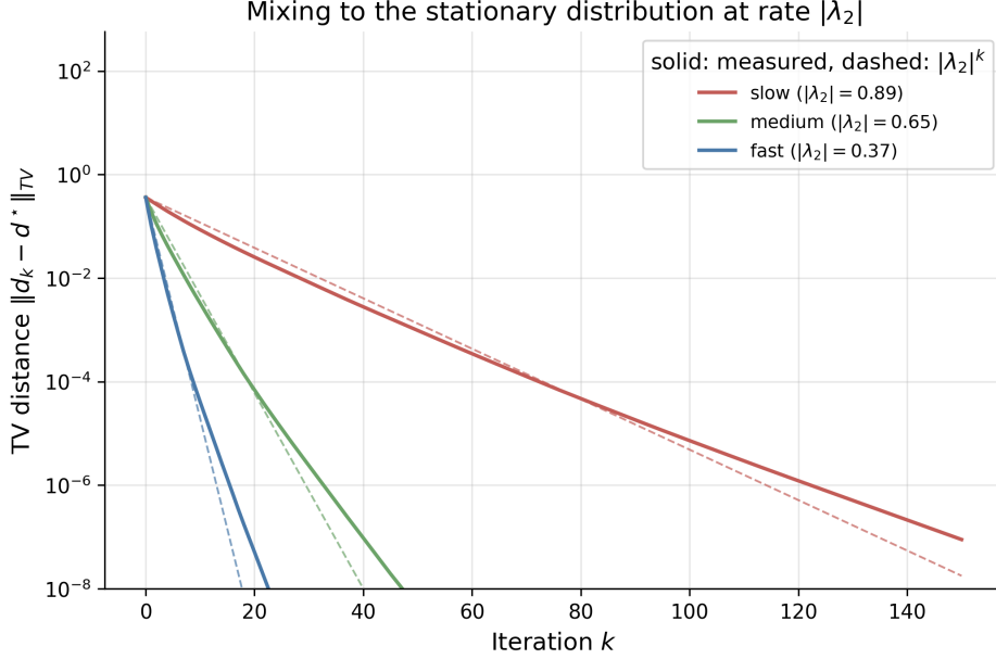
Figure 53: Total-variation distance \|d_k - d^*\|_{TV} of the state distribution d_k = d_0 P^k from the stationary distribution, on random 8-state chains at three mixing speeds, averaged over 30 seeds, on a log scale. The solid curves show the measured distance and the dashed curves the |\lambda_2|^k rate of Theorem 23, anchored at the seed-averaged |\lambda_2| as an illustrative reference rather than a per-chain bound.
