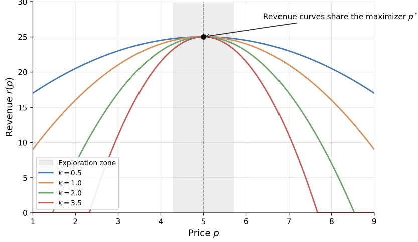
Figure 23: Revenue curves r(p) = r^* - k(p - p^*)^2 for four demand curvatures k \in \{0.5, 1.0, 2.0, 3.5\} . All revenue curves share the maximizer p^* = 5 ; the underlying demand curves (not shown here, see Broder and Rusmevichientong (2012) Theorem 3.1) are linearly distinct but cross at p^* . Within the illustrative exploration window |p - p^*| \leq 0.7 (shaded; half-width is pedagogical, not derived), revenue separation across the four curves is at most 1.72 units, about 7% of r^* , which is small relative to typical purchase-noise variance at this scale.
