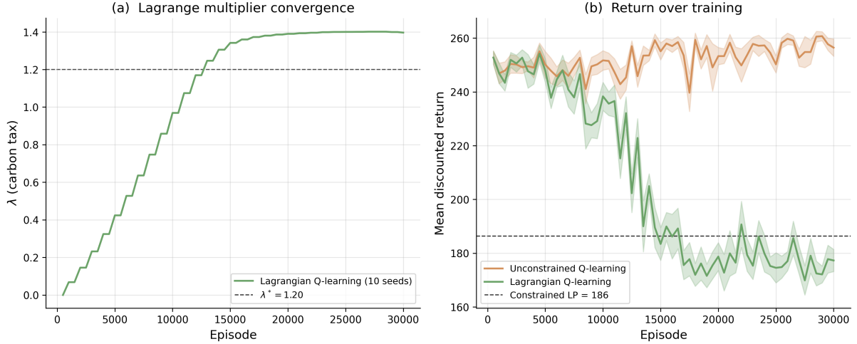
Figure 41: (a) Lagrange multiplier \lambda over training episodes, with the LP shadow price \lambda^* as the dashed reference. (b) Mean discounted return for unconstrained and Lagrangian Q-learning, with the constrained LP optimum as the dashed reference. Solid lines are means over ten seeds; shaded bands are \pm 1 standard error.
