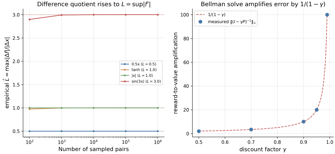
Figure 59: Left: the empirical Lipschitz constant \hat{L} , the largest difference quotient |f(x) - f(y)|/|x - y| over sampled pairs, approaching the analytic L = \sup |f'| (dashed) from below for four scalar functions, on a log-scaled pair count; the two piecewise-linear cases ( 0.5x , |x| ) sit at L already at the smallest sample size. Right: the reward-to-value amplification \|(I - \gamma P)^{-1}\|_\infty of the policy-evaluation solve against the discount factor \gamma (markers), matching 1/(1 - \gamma) (dashed).
