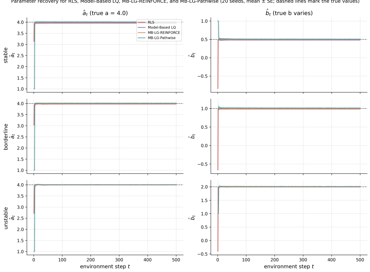
Figure 46: Parameter recovery for recursive least squares, the model-based LQ learner, and the MB-LG-REINFORCE and MB-LG-Pathwise ensemble means across stability regimes. Solid lines are means and shaded bands one standard error across twenty seeds; dashed horizontal lines mark the true values of a and b . All four methods converge to the truth within a few dozen environment steps.
