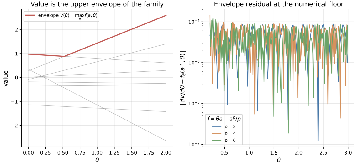
Figure 58: Left: a family of linear payoffs f(a, \theta) = \alpha_a + \beta_a \theta (thin) and their upper envelope V(\theta) = \max_a f(a, \theta) (thick), which coincides with the active member on each segment and kinks where the maximizer switches. Right: the envelope residual |dV/d\theta - \partial_\theta f(a^*, \theta)| against \theta for the smooth families f = \theta a - a^p/p , p \in \{2, 4, 6\} , on a log scale, at the finite-difference and grid-quantization floor.
