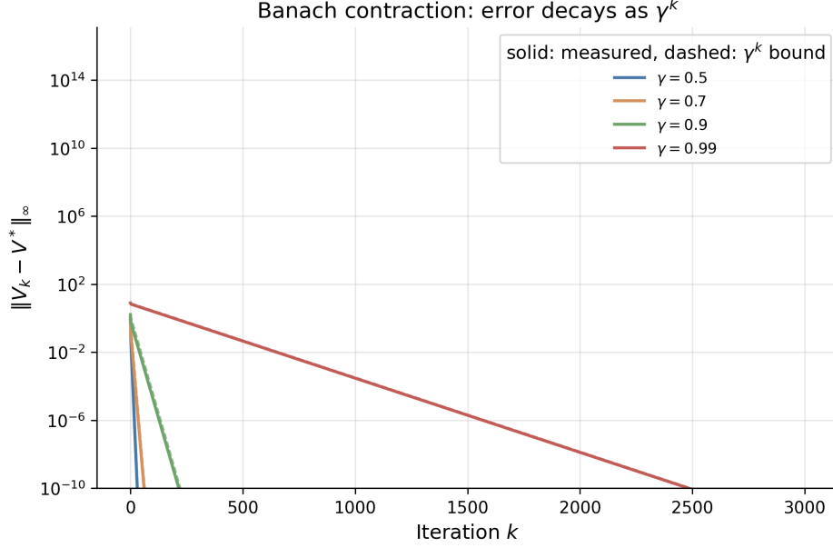
Figure 60: Supremum-norm error \|V_k - V^*\|_\infty of the iterates of the policy-evaluation operator T^\pi V = r^\pi + \gamma P^\pi V on random 50-state Markov reward processes, averaged over 30 seeds, on a log scale. The solid curves show the measured error and the dashed curves the \gamma^k \|V_0 - V^*\|_\infty bound of Theorem 28.
