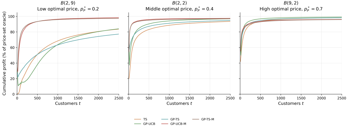
Figure 26: Weaver-style curve-learning pricing simulation across low, middle, and high optimal-price locations ( K = 10 , T = 2,500 , 1,000 seeds, price updates every 10 customers). The y -axis is cumulative profit divided by the price-set oracle. GP-UCB and GP-TS share information across nearby prices; GP-UCB-M and GP-TS-M additionally impose D'(p) \leq 0 through derivative-constrained GP curves. Shaded regions are \pm 2 standard errors.
