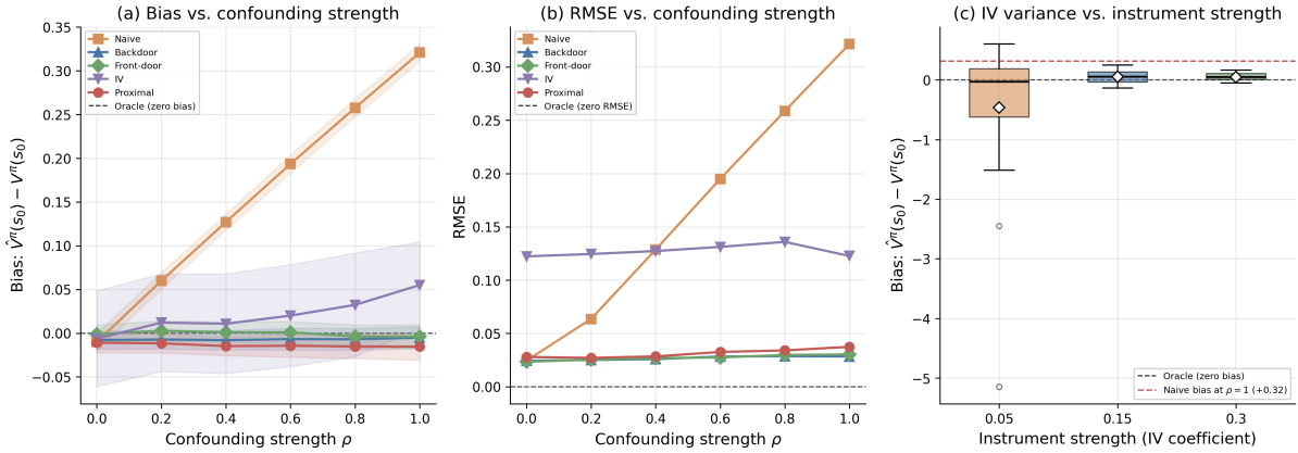
Figure 35: (a) Bias of five OPE estimators as a function of confounding strength \rho . (b) RMSE of five estimators as a function of \rho . (c) IV estimator bias distribution vs. instrument strength at \rho = 1 ; dashed red line is naive estimator bias.
