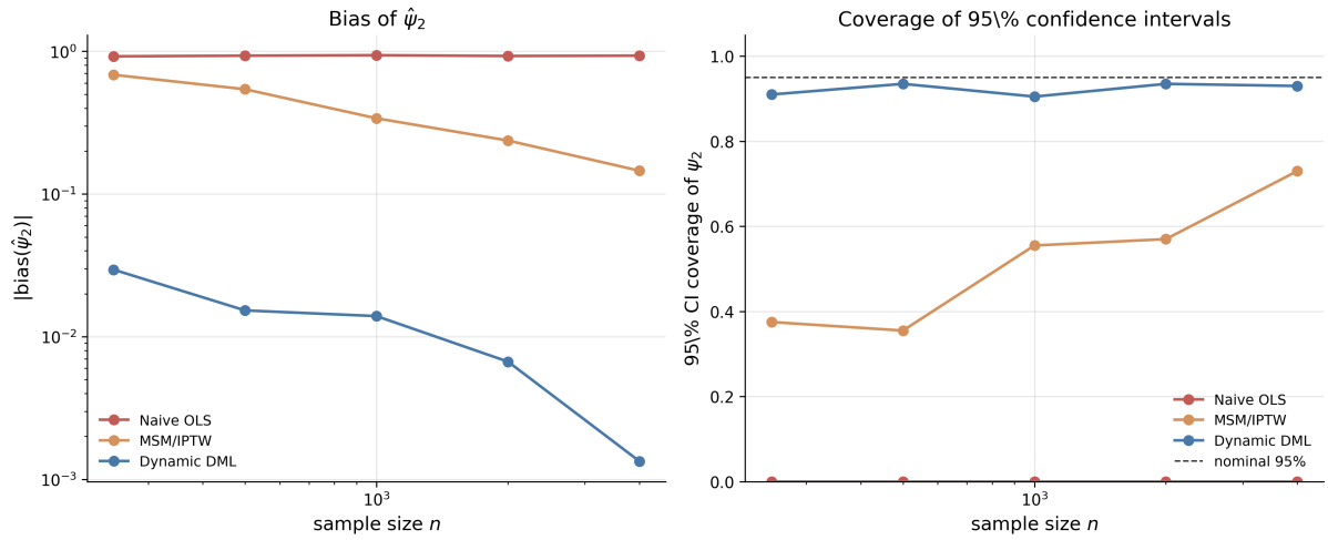
Figure 38: Sim 1, dynamic DML on a two-stage SNMM. Left panel: absolute bias of \hat{\psi}_2 versus sample size n (log-log). Right panel: empirical coverage of nominal 95% confidence intervals on \psi_2 versus n . Dotted reference line is the nominal coverage level. Each point averages 200 Monte Carlo replications under the data-generating process in Equation (168).
