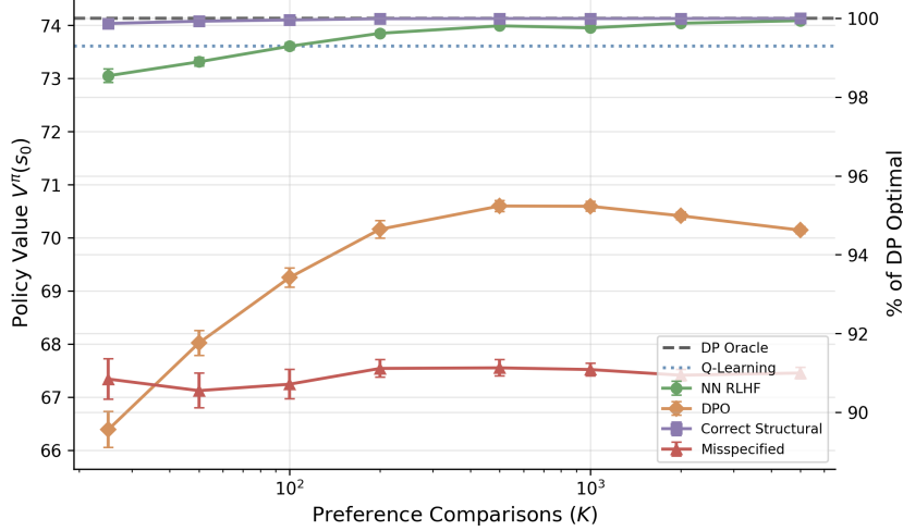
Figure 31: Policy value V^\pi(s_0) versus number of preference comparisons K for all six methods (30 seeds, L = 15 ). The right axis shows the percentage of DP-optimal value.
