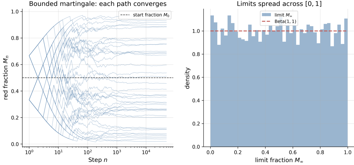
Figure 55: Left: the red-ball fraction M_n of a Pólya urn from a (1, 1) start against the step n on a log scale, for 40 seeds. Each bounded path converges to its own random limit. Right: the histogram of the limiting fractions across the ensemble, with the Beta(1, 1) density (dashed), the uniform law the theory predicts for this start.
