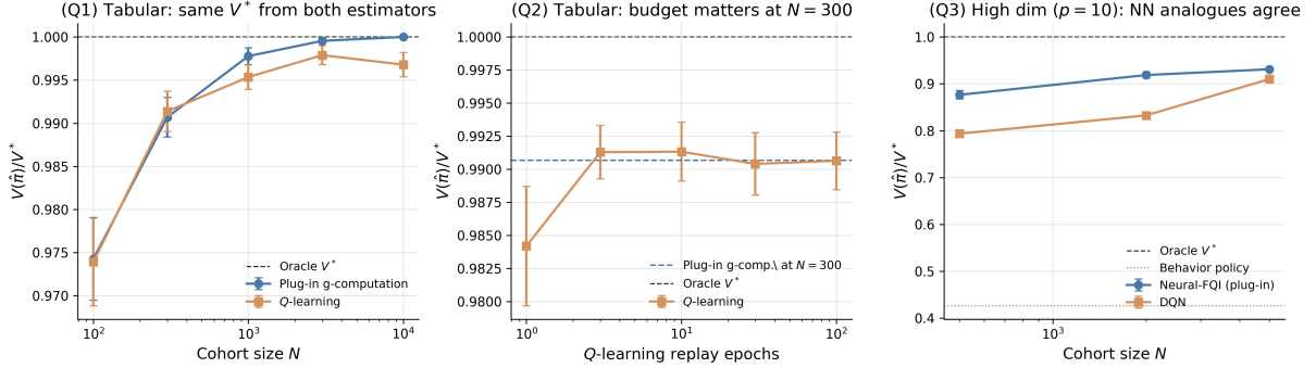
Figure 37: Plug-in g-computation (Murphy 2003 reference baseline) vs online Q -learning on a synthetic two-stage DTR under sequential ignorability. (Q1) Tabular sample-size sweep at fixed Q -learning budget, 50 Monte Carlo seeds, paired across estimators (both methods see the same cohort at each seed). (Q2) Tabular training-budget sweep at fixed N = 300 , 50 seeds, with the plug-in-g-computation converged value as the dashed reference. (Q3) High-dimensional sweep ( p = 10 continuous state), 20 seeds, paired across estimators, comparing Neural Fitted Q -Iteration to DQN with the same MLP architecture; the dotted line is the behavior-policy value. Error bars are 95% confidence intervals over Monte Carlo seeds.
