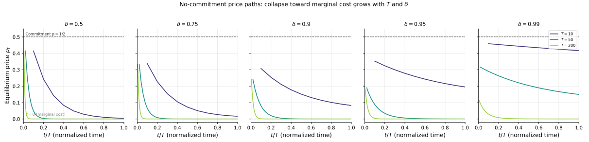
Figure 21: No-commitment price paths p_t versus normalized period t/T for representative horizons T \in \{10, 50, 200\} at \delta \in \{0.5, 0.75, 0.9, 0.95, 0.99\} . Dashed line: commitment price p = 1/2 . Dotted line: marginal cost c = 0 .
