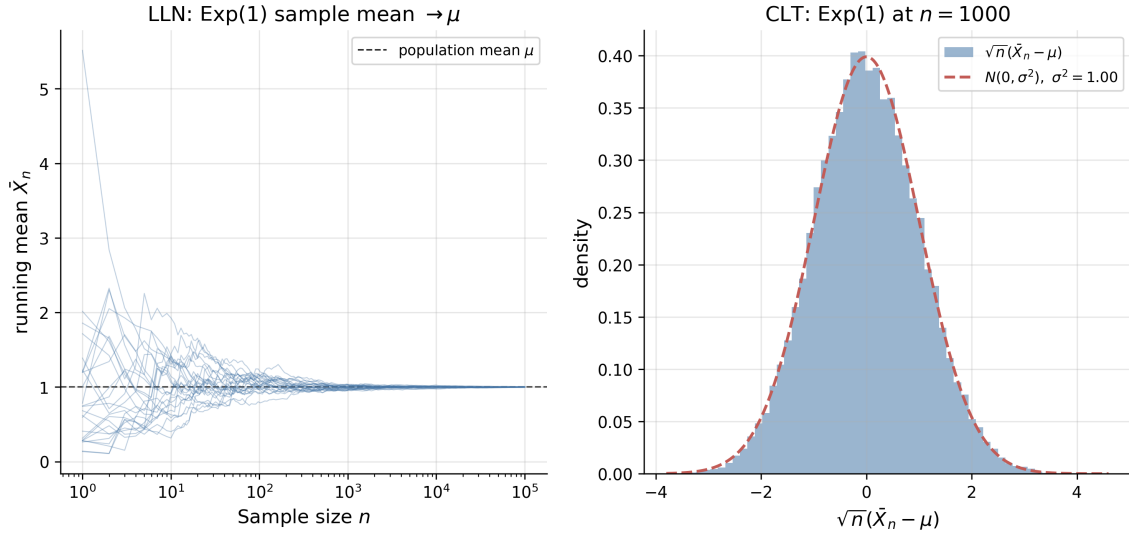
Figure 54: Left: running sample mean \bar{X}_n of \text{Exp}(1) draws against n on a log scale, for 25 seeds, converging to the population mean \mu = 1 (dashed). Right: histogram of the rescaled fluctuation \sqrt{n}(\bar{X}_n - \mu) for \text{Exp}(1) at n = 1000 over 40,000 replicates, with the N(0, \sigma^2) density overlaid (dashed).
