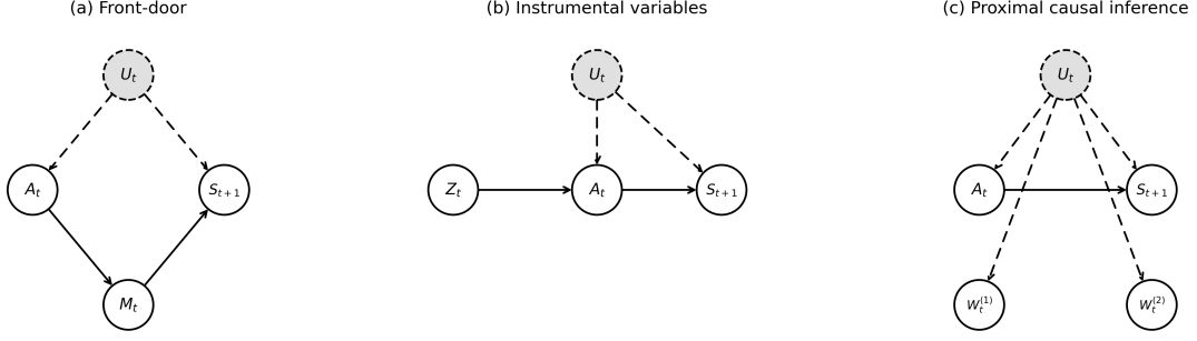
Figure 33: Causal graphs for three identification strategies in confounded MDPs. Gray dashed nodes are unobserved; dashed edges involve unobserved variables. (a) Front-door criterion with mediator M_t . (b) Instrumental variables with exogenous instrument Z_t . (c) Proximal causal inference with proxies W_t^{(1)}, W_t^{(2)} .
