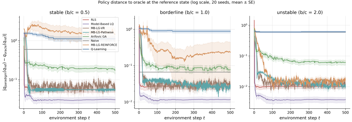
Figure 47: Policy distance to the oracle at a regime-specific reference state, log scale. The reference state is the static optimum quantity for each regime. Lines are means and bands one standard error across twenty seeds. Oracle is identically zero by construction and is omitted.
