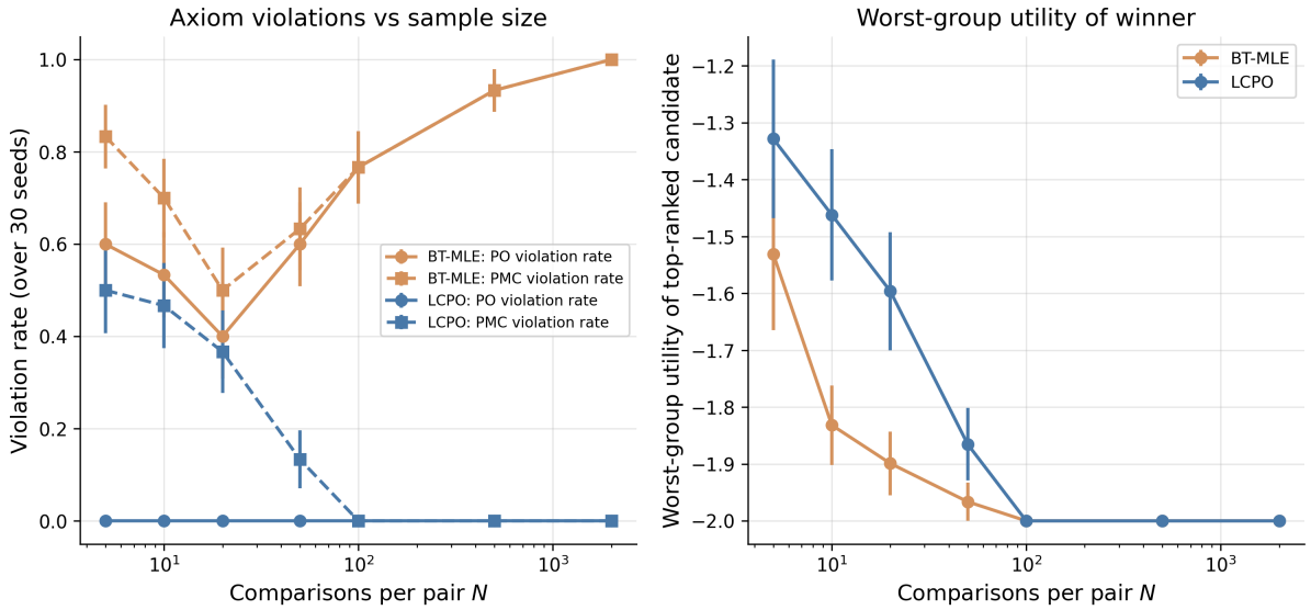
Figure 29: Axiom violation rates (left) and worst-group utility of the top-ranked candidate (right) versus pairwise comparisons per pair N , mean and one standard error over thirty seeds. BT-MLE PO and PMC violation rates rise to one as N grows, in line with Theorem 14; LCPO violation rates remain at zero (PO by construction) or fall to zero (PMC by N = 100 ).
