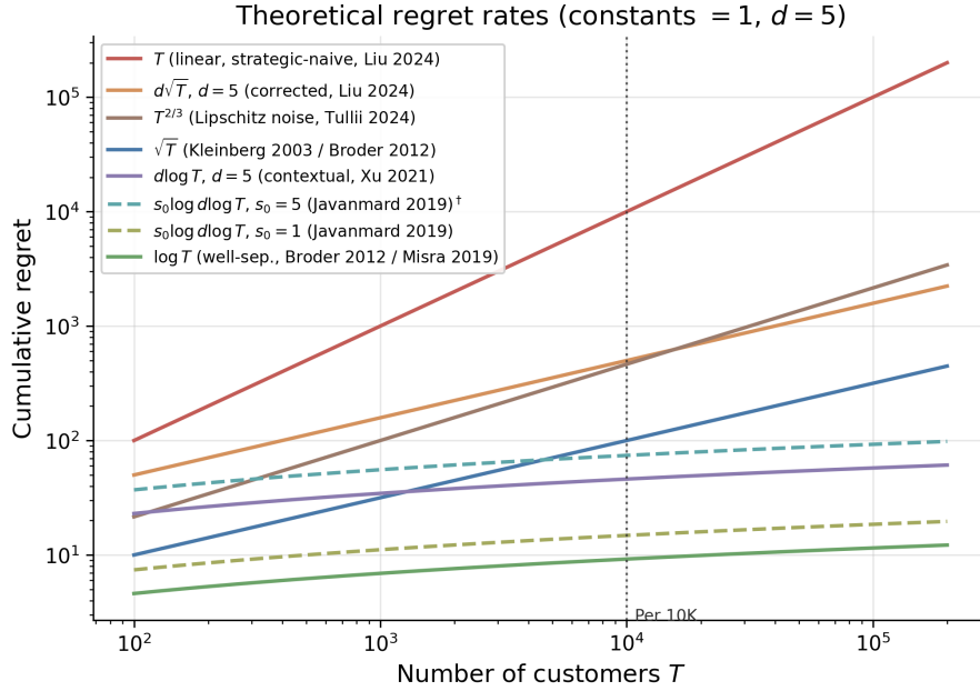
Figure 24: Theoretical regret rate functions at constants equal to 1, d = 5 . Legend names the source paper for each rate. Two cases for the s_0 \log d \log T rate are shown: s_0 = 1 (very sparse, \approx 15 lost at T = 10,000 ) and s_0 = 5 (here s_0 = d , \approx 74 lost), which at this constants-equal-to-1 calibration sits above d \log T because s_0 \log d \approx 8.0 > d = 5 ; sparse dominates when s_0 \ll d . The vertical line marks T = 10,000 , matching the “Per 10K” column of Table 24.
