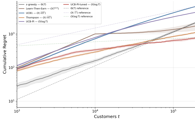
Figure 25: Cumulative regret on log-log axes ( K = 100 , S = 1,000 , 10 seeds). Each algorithm’s legend entry includes its theoretical regret rate. Dashed lines show \Theta(T) , O(\sqrt{T}) , and O(\log T) reference rates. Shaded regions are \pm 2 standard errors.
