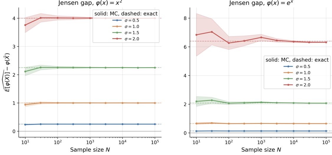
Figure 53: Plug-in Monte Carlo estimate of the Jensen gap \mathbb{E}[\varphi(X)] - \varphi(\mathbb{E}[X]) for X \sim N(0, \sigma^2) against sample size N , for \varphi(x) = x^2 (left) and \varphi(x) = e^x (right), at four values of \sigma , averaged over 40 seeds with a \pm 1 standard-error band. The dashed lines are the closed-form gaps \sigma^2 and e^{\sigma^2/2} - 1 . The solid line at zero marks the sign floor the inequality forbids the gap to cross.
