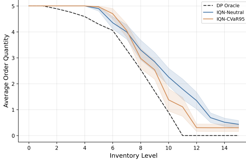
Figure 40: Average order quantity by inventory level for the DP oracle and the two IQN evaluation policies. Mean across ten training seeds with \pm 1 SE bands, 50,000 evaluation episodes per seed.
