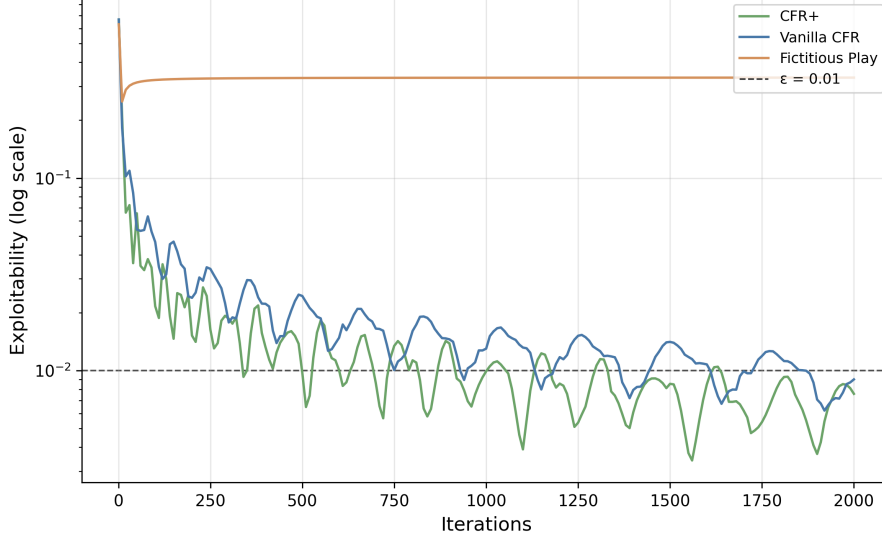
Figure 20: Exploitability versus iteration (log scale) for CFR+, vanilla CFR, and fictitious play in Kuhn poker. The dashed reference line marks \varepsilon = 0.01 .
