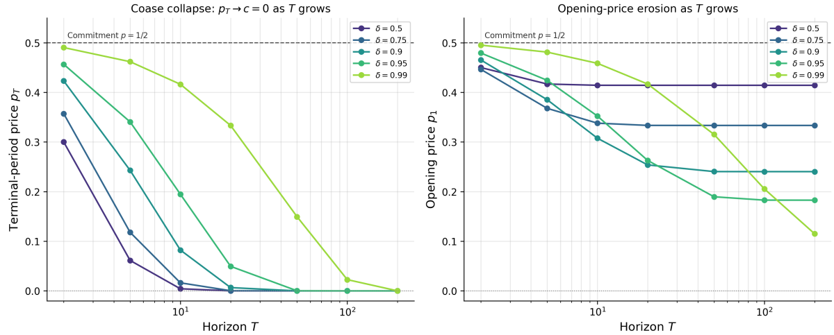
Figure 22: Coase collapse. Left: terminal-period price p_T versus T on a log- T axis. Right: opening price p_1 versus T , same axis. Each curve fixes \delta .
