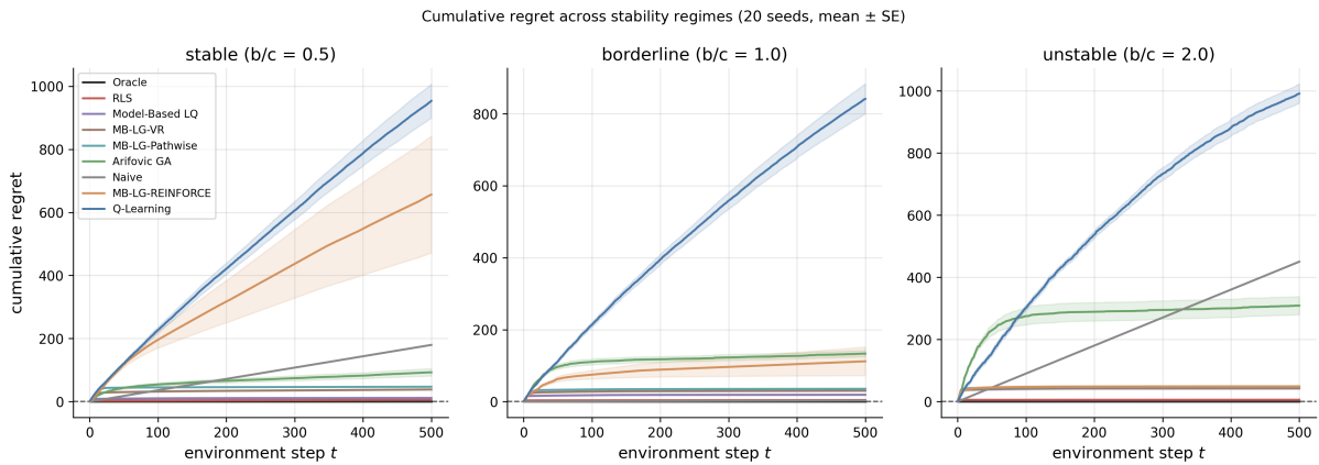
Figure 45: Cumulative regret across stability regimes for nine learning paradigms on the cobweb with adjustment cost. Lines are means and shaded bands are one standard error across twenty seeds. Panels correspond to b/c \in \{0.5, 1.0, 2.0\} . Oracle is the zero reference.
