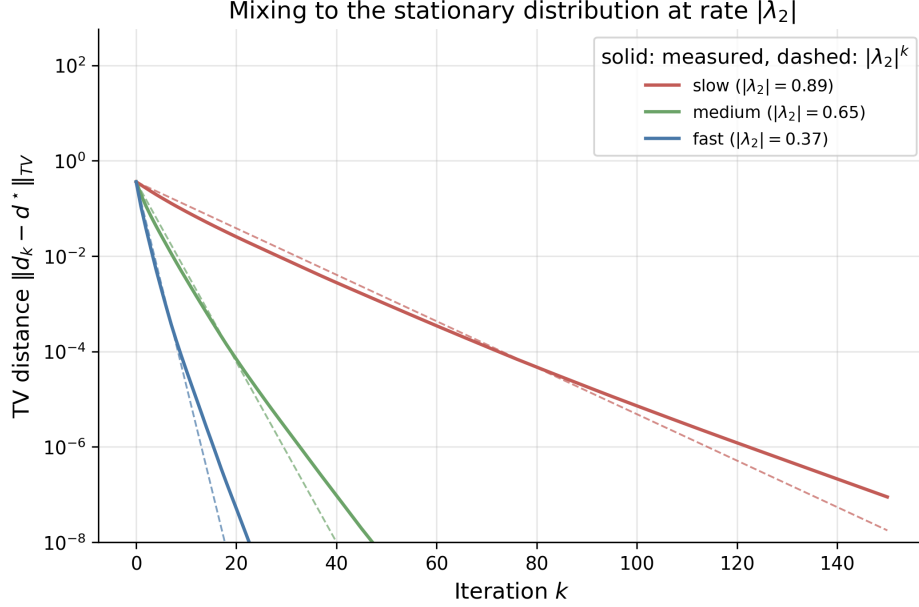
Figure 51: Total-variation distance \|d_k - d^*\|_{TV} of the state distribution d_k = d_0 P^k from the stationary distribution, on random 8-state chains at three mixing speeds, averaged over 30 seeds, on a log scale. The solid curves show the measured distance and the dashed curves the |\lambda_2|^k rate of Theorem 19, anchored at the seed-averaged |\lambda_2| as an illustrative reference rather than a per-chain bound.
