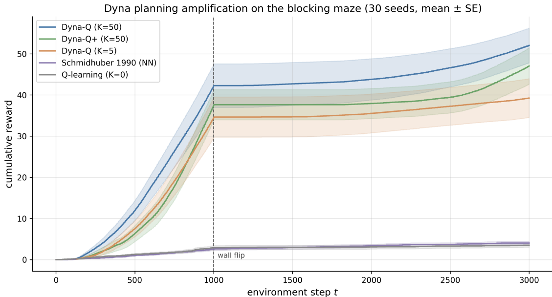
Figure 44: Cumulative reward on the blocking maze for five agents under a shared three-thousand-step environment budget. The dashed vertical line marks the wall flip at t = 1000 . Lines are means and shaded bands are one standard error across thirty seeds.
