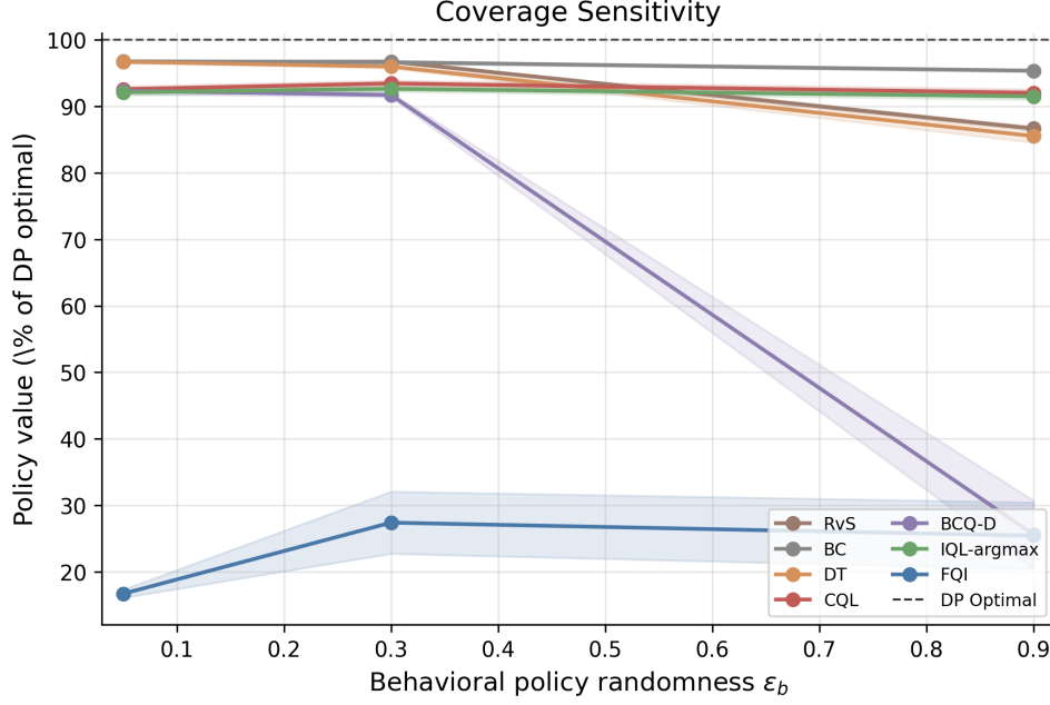
Figure 27: Policy value (as % of DP optimal) versus behavioral policy randomness \epsilon_b for the value-based methods (FQI, CQL, IQL-argmax, BCQ-D), the supervised-conditioning family (DT, RvS), and the behavioral cloning baseline (BC). Higher \epsilon_b increases data coverage.
