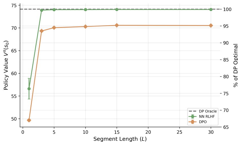
Figure 32: Policy value V^\pi(s_0) versus segment length L at K = 2,000 for the neural network and DPO (20 seeds). The right axis shows the percentage of DP-optimal value.
