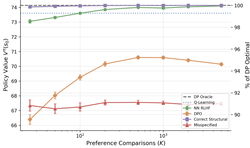
Figure 18: Policy value V^\pi(s_0) versus number of preference comparisons K for all six methods (30 seeds, L = 15 ). The right axis shows the percentage of DP-optimal value.
