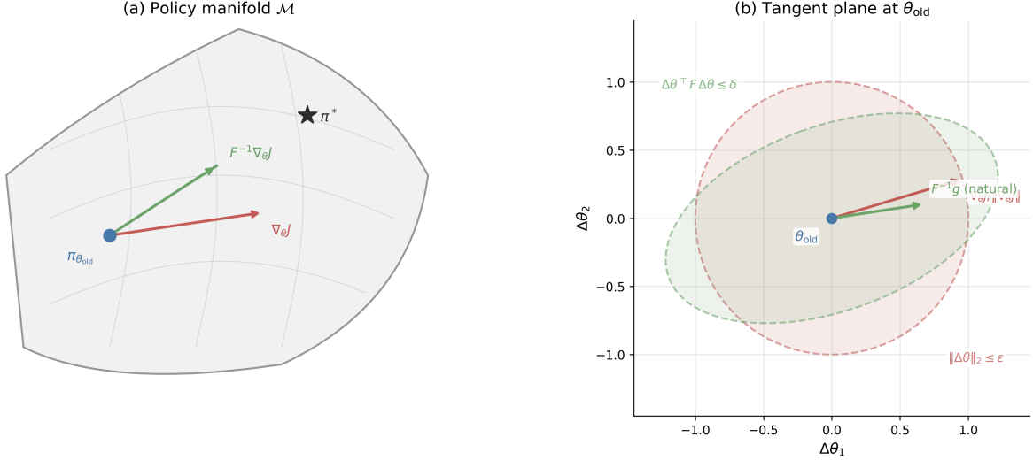
Figure 9: Information geometry of the natural policy gradient. Left : the policy manifold \mathcal{M} with Euclidean gradient \nabla_{\theta} J (red) and natural gradient F^{-1}\nabla_{\theta} J (green) from the current iterate \pi_{\theta_{\text{old}}} toward the optimal policy \pi^* . Right : tangent plane at \theta_{\text{old}} showing the Euclidean unit ball \|\Delta\theta\|_2 \leq \epsilon (red) and the KL unit ball \Delta\theta^\top F \Delta\theta \leq \delta (green), with the respective steepest-ascent directions.
