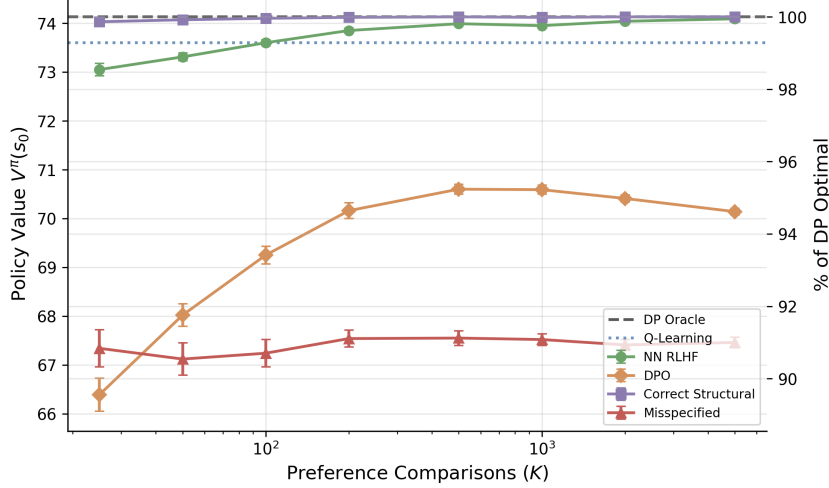
Figure 27: Policy value V^\pi(s_0) versus number of preference comparisons K for all six methods (30 seeds, L = 15 ). The right axis shows the percentage of DP-optimal value.
