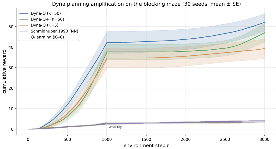
Figure 39: Cumulative reward on the blocking maze for five agents under a shared three-thousand-step environment budget. The dashed vertical line marks the wall flip at t = 1000 . Lines are means and shaded bands are one standard error across thirty seeds.
