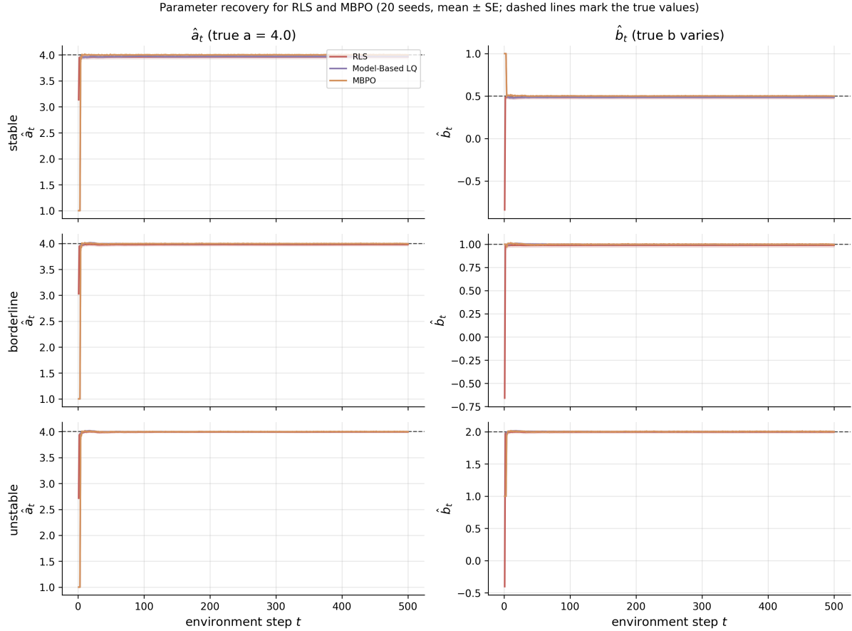
Figure 41: Parameter recovery for recursive least squares, the model-based LQ learner, and the MBPO ensemble mean across stability regimes. Solid lines are means and shaded bands one standard error across twenty seeds; dashed horizontal lines mark the true values of a and b . All three methods converge to the truth within a few dozen environment steps.
