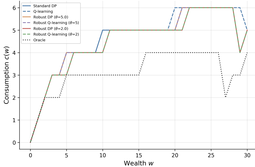
Figure 37: Consumption policy c(w) for each method. Dashed lines show Q-learning policies; solid lines show DP.
