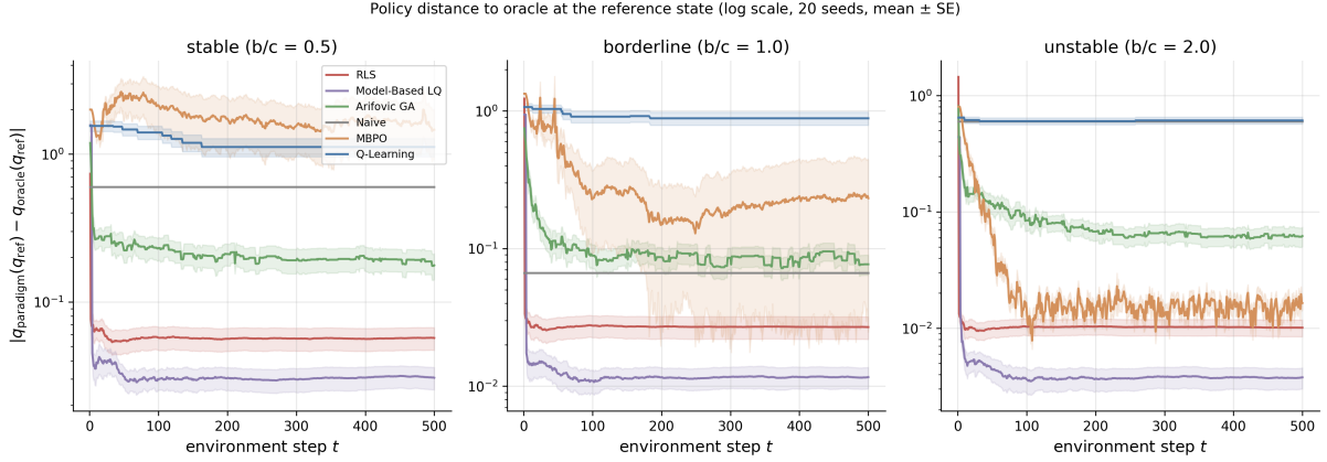
Figure 42: Policy distance to the oracle at a regime-specific reference state, log scale. The reference state is the static optimum quantity for each regime. Lines are means and bands one standard error across twenty seeds. Oracle is identically zero by construction and is omitted.
