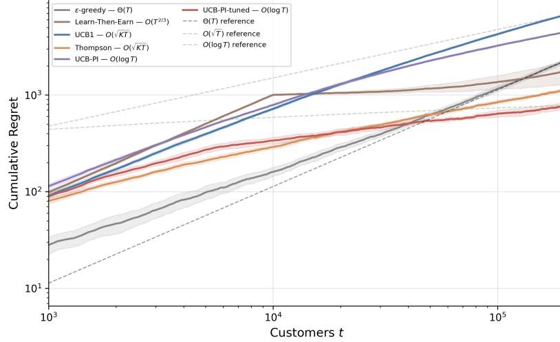
Figure 22: Cumulative regret on log-log axes ( K = 100 , S = 1,000 , 10 seeds). Each algorithm’s legend entry includes its theoretical regret rate. Dashed lines show \Theta(T) , O(\sqrt{T}) , and O(\log T) reference rates. Shaded regions are \pm 2 standard errors.
