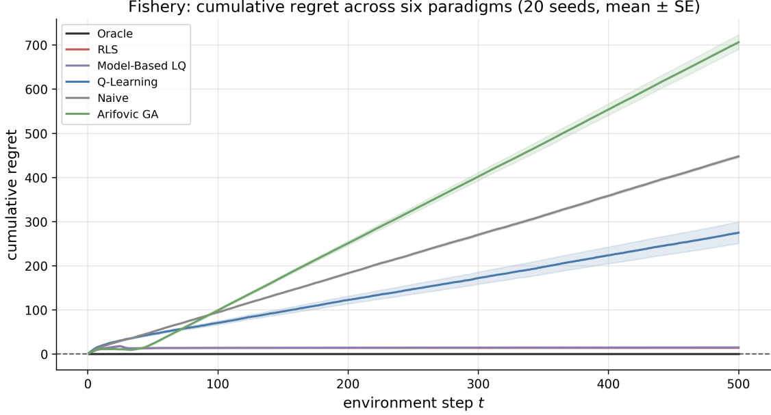
Figure 43: Cumulative regret on the logistic-growth fishery for six paradigms (twenty seeds, mean and one-standard-error bands). Paradigms are presented in rank order by final regret.
