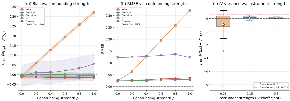
Figure 31: (a) Bias of five OPE estimators as a function of confounding strength \rho . (b) RMSE of five estimators as a function of \rho . (c) IV estimator bias distribution vs. instrument strength at \rho = 1 ; dashed red line is naive estimator bias.
