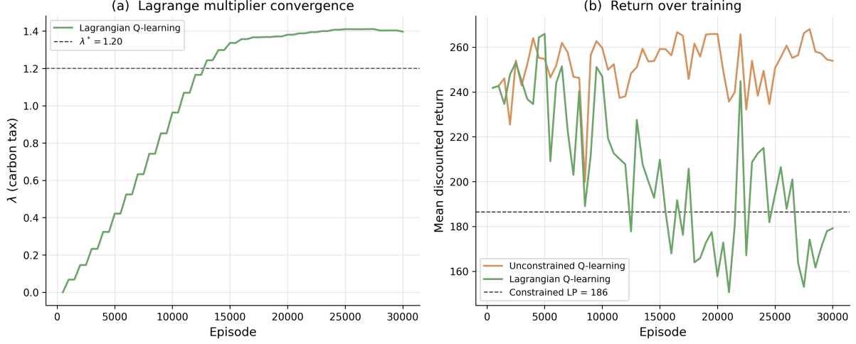
Figure 36: (a) Lagrange multiplier \lambda over training episodes, with the LP shadow price \lambda^* as the dashed reference. (b) Mean discounted return for unconstrained and Lagrangian Q-learning, with the constrained LP optimum as the dashed reference.
