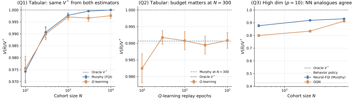
Figure 33: Murphy’s batch backward regression vs online Q -learning on a synthetic two-stage DTR under sequential ignorability. (Q1) Tabular sample-size sweep at fixed Q -learning budget. (Q2) Tabular training-budget sweep at fixed N = 300 , with Murphy’s converged value as the dashed reference. (Q3) High-dimensional sweep ( p = 10 continuous state), comparing Neural Fitted Q -Iteration to DQN with the same MLP architecture; the dotted line is the behavior-policy value. Error bars are 95% confidence intervals over Monte Carlo seeds.
