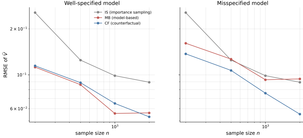
Figure 32: Root mean squared error of three OPE estimators against the sample size, log-log scale, two panels. Left panel, well-specified outcome model. Right panel, misspecified model with the interaction omitted. The MB estimator’s RMSE plateaus under misspecification as the bias dominates the variance, while the CF estimator’s RMSE continues to decline.
