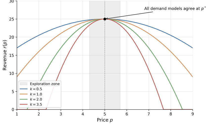
Figure 20: Revenue curves r(p) = r^* - k(p - p^*)^2 for four demand curvatures k \in \{0.5, 1.0, 2.0, 3.5\} . All models agree at the optimal price p^* = 5 . Within the shaded exploration zone, the curves are nearly indistinguishable, so playing prices near p^* is uninformative about the demand parameter.
