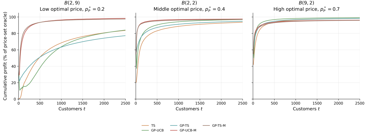
Figure 23: Weaver-style curve-learning pricing simulation across low, middle, and high optimal-price locations ( K = 10 , T = 2,500 , 1,000 seeds, price updates every 10 customers). The y -axis is cumulative profit divided by the price-set oracle. GP-UCB and GP-TS share information across nearby prices; GP-UCB-M and GP-TS-M additionally impose D'(p) \leq 0 through derivative-constrained GP curves. Shaded regions are \pm 2 standard errors.
