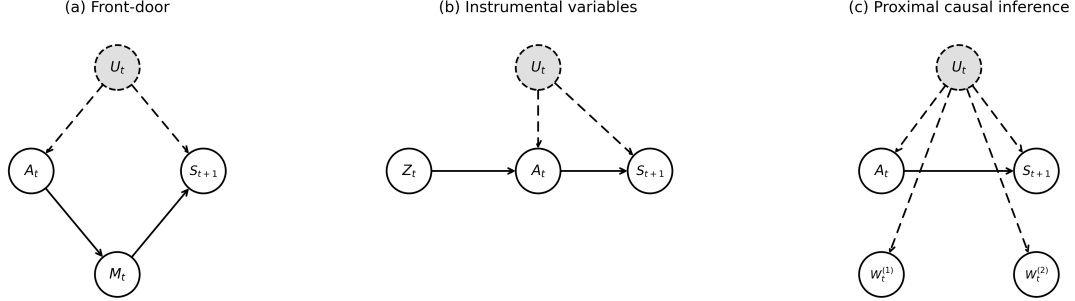
Figure 29: Causal graphs for three identification strategies in confounded MDPs. Gray dashed nodes are unobserved; dashed edges involve unobserved variables. (a) Front-door criterion with mediator M_t . (b) Instrumental variables with exogenous instrument Z_t . (c) Proximal causal inference with proxies W_t^{(1)}, W_t^{(2)} .
