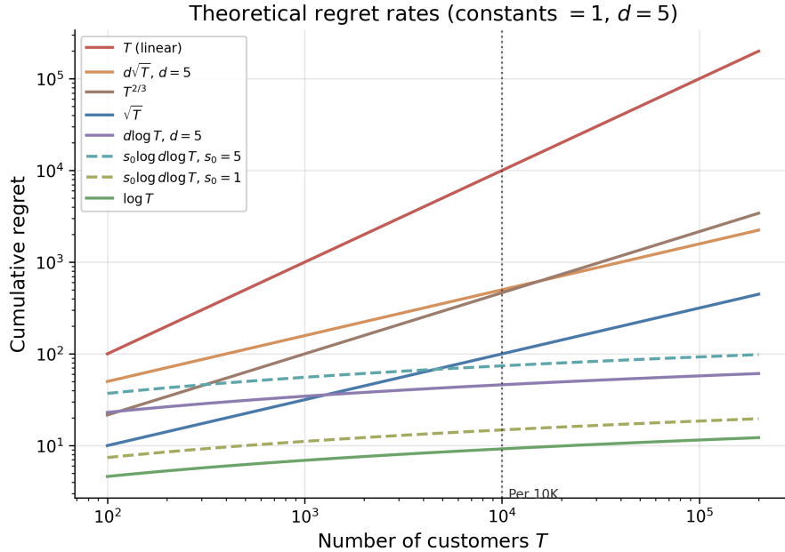
Figure 21: Theoretical regret rate functions at constants equal to 1, d = 5 . Two cases for the s_0 \log d \log T rate are shown: s_0 = 1 (very sparse, \approx 15 lost at T = 10,000 ) and s_0 = 5 (moderate sparsity, \approx 74 lost). The vertical line marks T = 10,000 , matching the “Per 10K” column of Table 21.
