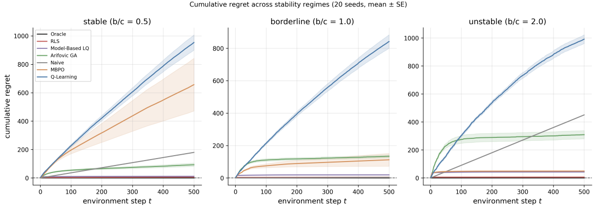
Figure 40: Cumulative regret across stability regimes for seven learning paradigms on the cobweb with adjustment cost. Lines are means and shaded bands are one standard error across twenty seeds. Panels correspond to b/c \in \{0.5, 1.0, 2.0\} . Oracle is the zero reference.
