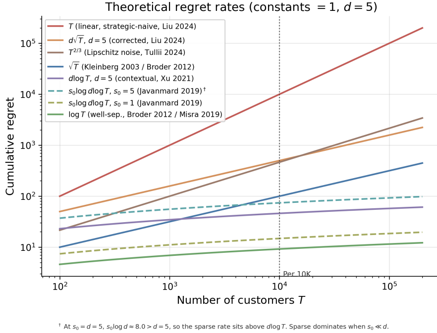
Figure 25: Theoretical regret rate functions at constants equal to 1, d = 5 . Legend names the source paper for each rate. Two cases for the s_0 \log d \log T rate are shown: s_0 = 1 (very sparse, \approx 15 lost at T = 10,000 ) and s_0 = 5 (here s_0 = d , \approx 74 lost), which at this constants-equal-to-1 calibration sits above d \log T because s_0 \log d \approx 8.0 > d = 5 ; sparse dominates when s_0 \ll d . The vertical line marks T = 10,000 , matching the “Per 10K” column of Table 25.
