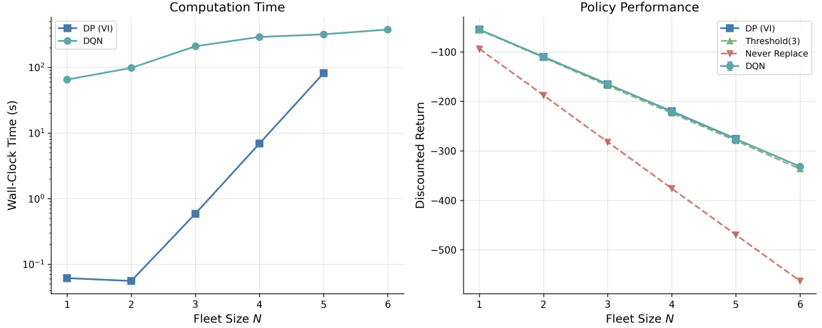
Figure 1: Bus engine replacement benchmark. Left: computation time vs. fleet size (log scale). Right: discounted return vs. fleet size for DP, DQN, and heuristic baselines. At N = 6 (46,656 states), DP is infeasible (no data point).
