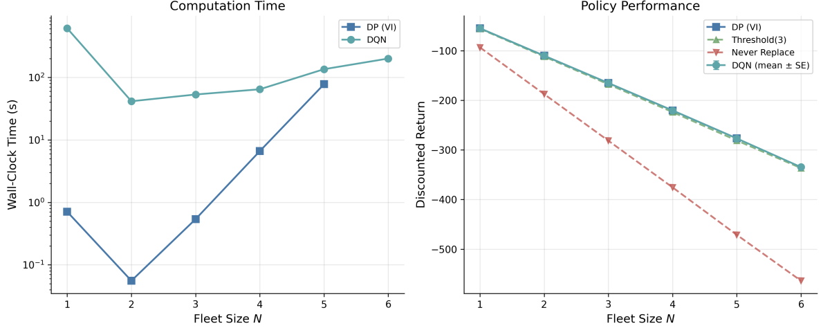
Figure 14: Bus engine replacement benchmark. Left: computation time vs. fleet size (log scale). Right: discounted return vs. fleet size for DP, DQN, and heuristic baselines; DQN error bars are mean \pm standard error over ten seeds. At N = 6 (46,656 states), DP is omitted because plain-Python value iteration becomes wall-clock prohibitive at this scale.
