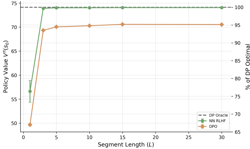
Figure 28: Policy value V^\pi(s_0) versus segment length L at K = 2,000 for the neural network and DPO (20 seeds). The right axis shows the percentage of DP-optimal value.
