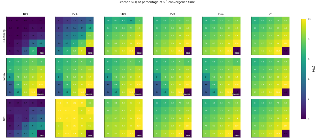
Figure 12: Learned value function V(s) at percentage-based checkpoints of each algorithm's V^* -convergence time T , defined as the first episode where \max_s |V(s) - V^*(s)| < 0.1 ; algorithms that never converge use T = 500,000 . All columns share the same color scale, so a converged algorithm's grid visually matches the V^* reference column. Off-policy methods (Q-learning, Q( \lambda ), DQN) converge to V^* everywhere. On-policy methods (SARSA, REINFORCE, NPG, PPO) show persistent discrepancies at off-path states even at the final episode.
