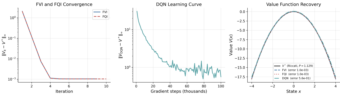
Figure 4: LQC convergence of FVI and FQI (left), DQN learning curve (middle), and value function recovery for all three methods (right). FVI and FQI reduce \|V_k - V^*\|_\infty to near-zero in under 10 iterations, exploiting the known polynomial structure of Q^* . DQN declines from error 6.7 to 0.56 over 100,000 gradient steps with no feature basis specified.
