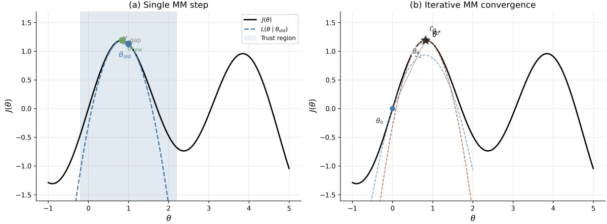
Figure 8: Majorization-minimization interpretation of trust region updates. Left : the surrogate L(\theta|\theta_{\text{old}}) (dashed) lower-bounds J(\theta) (solid) and is tight at \theta_{\text{old}} ; the trust region (shaded) constrains the step. The gap between L(\theta_{\text{new}}) and J(\theta_{\text{new}}) is the guaranteed improvement. Right : iterative MM convergence from \theta_0 through four surrogates (dashed, colored by iteration) to \theta^* .
