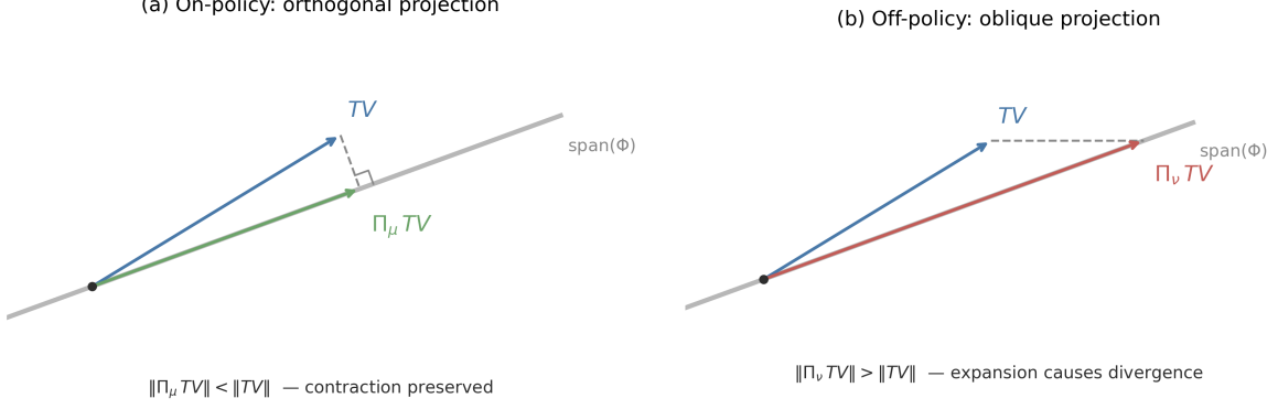
Figure 6: Geometry of the projected Bellman operator in \mathbb{R}^2 . The gray line is the function approximation subspace \text{span}(\Phi) ; the blue arrow is TV , the Bellman update. (a) On-policy: the orthogonal projection \Pi_\mu drops TV perpendicularly onto the subspace, preserving the contraction. (b) Off-policy: the oblique projection \Pi_\nu (under the behavior distribution) reaches a point further from the origin than TV itself, causing expansion.
