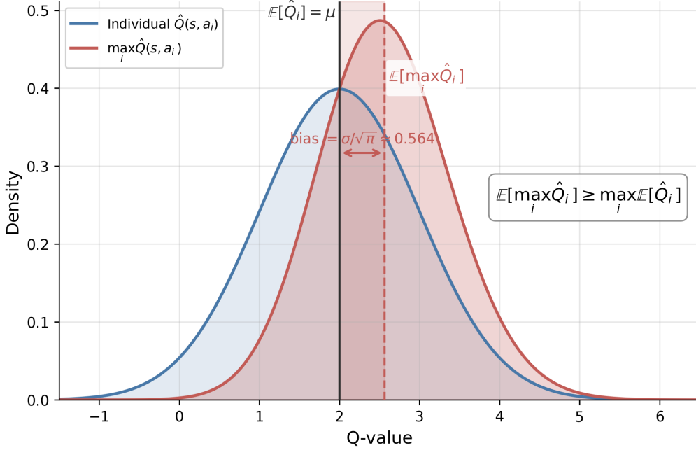
Figure 10: Overestimation bias from Jensen’s inequality with n = 2 actions. Blue: density of individual \hat{Q}(s, a_i) \sim \mathcal{N}(\mu, \sigma^2) . Red: density of \max_i \hat{Q}(s, a_i) , shifted right by \sigma/\sqrt{\pi} \approx 0.56 . The shaded gap is the bias. With n = 100 actions the bias exceeds 2.5\sigma .
