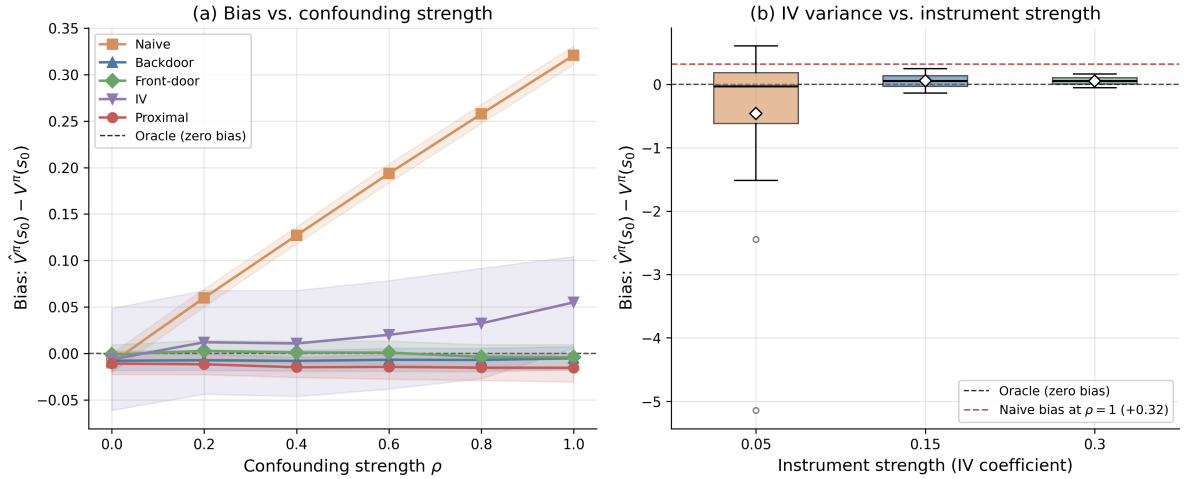
Figure 26: (a) Bias of five OPE estimators relative to the oracle as a function of confounding strength \rho . (b) IV estimator bias distribution vs. instrument strength at \rho = 1 . Dashed red line: naive estimator bias.
