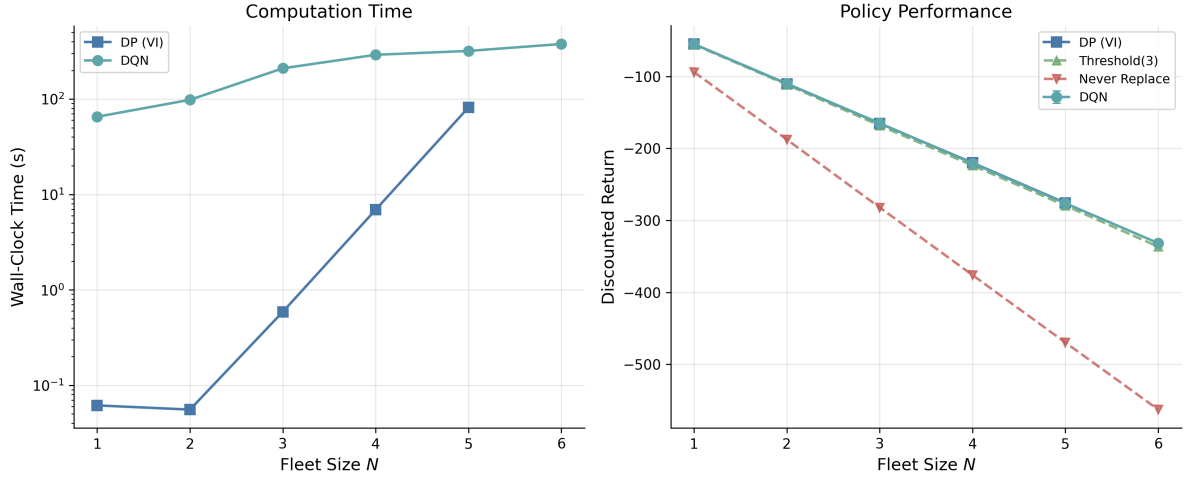
Figure 14: Bus engine replacement benchmark. Left: computation time vs. fleet size (log scale). Right: discounted return vs. fleet size for DP, DQN, and heuristic baselines.
