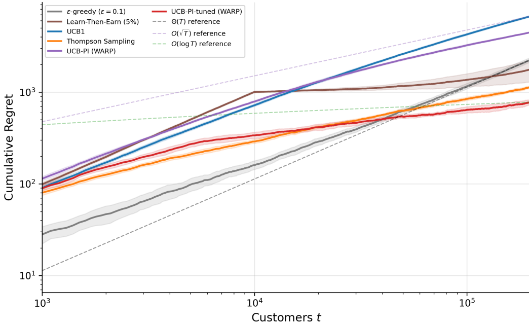
Figure 19: Cumulative regret on log-log axes. Dashed lines show \Theta(T) , O(\sqrt{T}) , and O(\log T) reference rates. Shaded regions are \pm 2 standard errors across 10 seeds.
