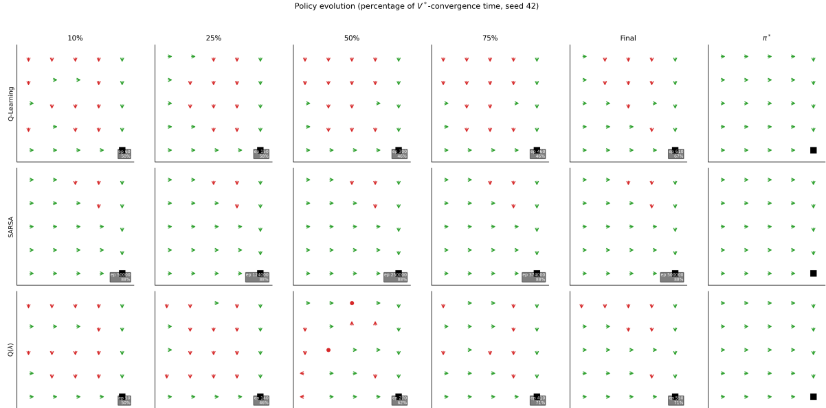
Figure 13: Policy grids at percentage-based checkpoints of V^* -convergence time T (same definition as Figure 12). Arrows indicate the greedy action at each state; dots indicate the stay action. Off-policy methods converge to \pi^* everywhere. On-policy methods retain incorrect actions at states far from the optimal path.
