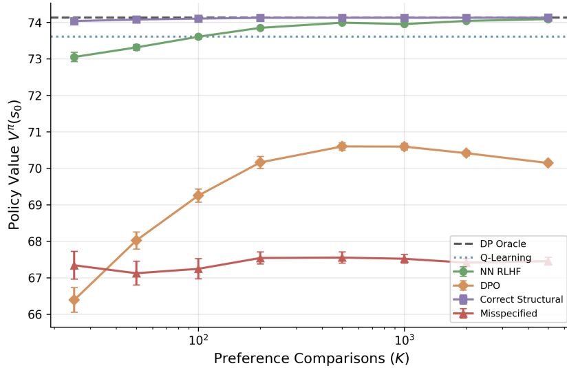
Figure 22: Policy value V^\pi(s_0) versus number of preference comparisons K for all six methods.
