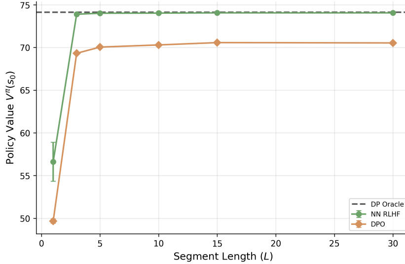
Figure 23: Policy value V^\pi(s_0) versus segment length L at K = 2,000 for the neural network and DPO.
