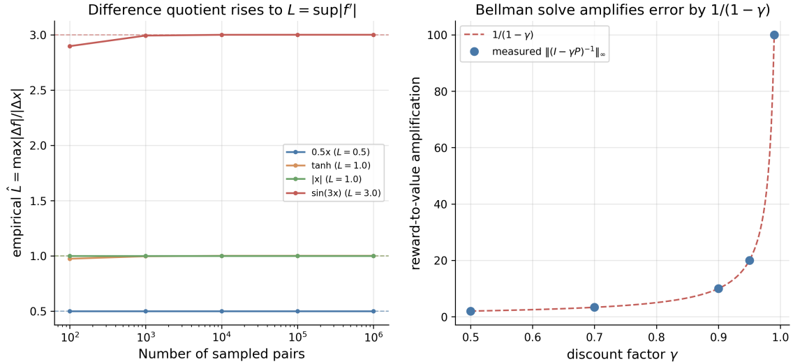
Figure 60: Left: the empirical Lipschitz constant \hat{L} , the largest difference quotient |f(x) - f(y)|/|x - y| over sampled pairs, approaching the analytic L = \sup |f'| (dashed) from below for four scalar functions, on a log-scaled pair count; the two piecewise-linear cases ( 0.5x , |x| ) sit at L already at the smallest sample size. Right: the reward-to-value amplification \|(I - \gamma P)^{-1}\|_\infty of the policy-evaluation solve against the discount factor \gamma (markers), matching 1/(1 - \gamma) (dashed).
