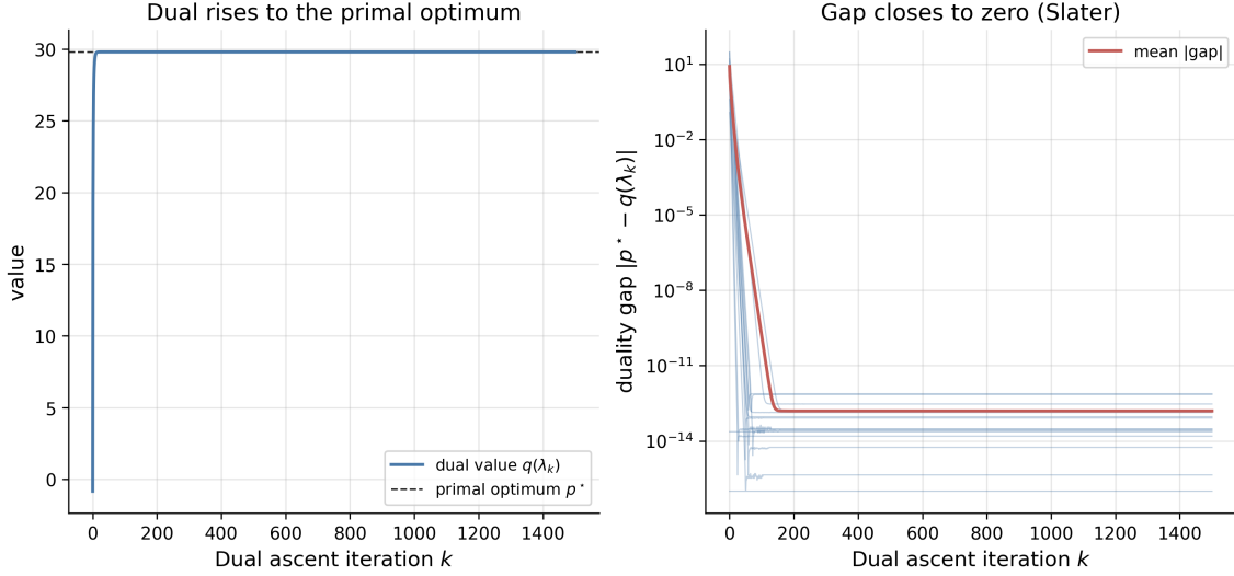
Figure 58: Left: dual value g(\lambda_k) of a convex quadratic program under projected dual ascent, rising to the primal optimum p^* (dashed) from below. Right: the duality gap |p^* - g(\lambda_k)| against the iteration, for 15 random instances (thin) and their mean (thick), on a log scale, closing to solver precision because a strictly feasible point exists.
