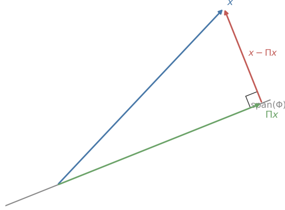
Figure 53: The orthogonal projection \Pi x of a point x onto a subspace. The residual x - \Pi x meets the subspace at a right angle, so the three vectors form a right triangle and \Pi x is a leg no longer than the hypotenuse x .
