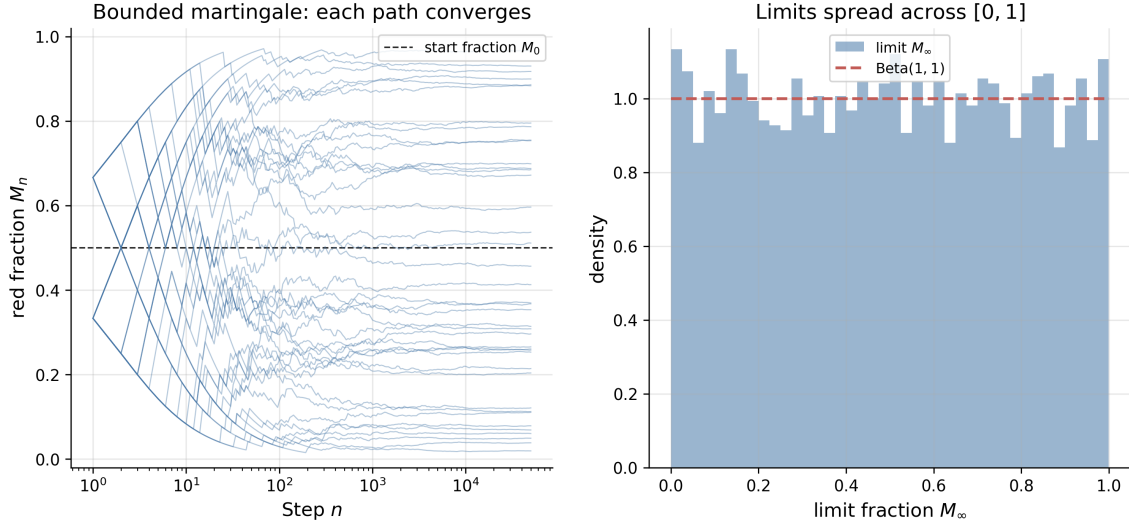
Figure 56: Left: the red-ball fraction M_n of a Pólya urn from a (1, 1) start against the step n on a log scale, for 40 seeds. Each bounded path converges to its own random limit. Right: the histogram of the limiting fractions across the ensemble, with the Beta(1,1) density (dashed), the uniform law the theory predicts for this start.
