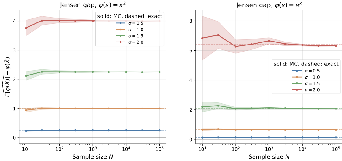
Figure 54: Plug-in Monte Carlo estimate of the Jensen gap \mathbb{E}[\varphi(X)] - \varphi(\mathbb{E}[X]) for X \sim N(0, \sigma^2) against sample size N , for \varphi(x) = x^2 (left) and \varphi(x) = e^x (right), at four values of \sigma , averaged over 40 seeds with a \pm 1 standard-error band. The dashed lines are the closed-form gaps \sigma^2 and e^{\sigma^2/2} - 1 . The solid line at zero marks the sign floor the inequality forbids the gap to cross.
