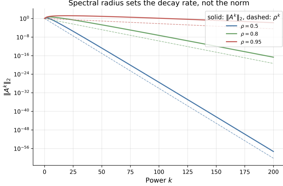
Figure 50: Operator norm \|A^k\|_2 of the powers of the non-normal matrix A = \begin{bmatrix} \rho & 2 \\ 0 & \rho \end{bmatrix} , on a log scale. The solid curves grow to a transient peak before decaying. The dashed curves are \rho^k . Both share the asymptotic slope, so \rho sets the decay rate even though \|A\|_2 > 1 .
