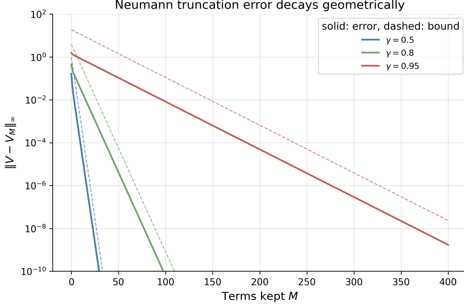
Figure 51: Supremum-norm error of truncating V = \sum_m \gamma^m P^m r at M terms, on random 40-state chains, averaged over 30 seeds, on a log scale. The solid curves show the measured error and the dashed curves the bound \gamma^{M+1} \|r\|_\infty / (1 - \gamma) of Theorem 22.
