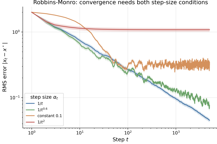
Figure 62: Root-mean-square error |x_t - x^*| of the stochastic-approximation recursion (213) for the fixed point of x = \gamma x + b under four step-size schedules, averaged over 100 seeds, on log-log axes. Only the two schedules that satisfy both Robbins-Monro conditions (214) reach the root. The constant schedule settles into a noise floor. The 1/t^2 schedule stalls.
