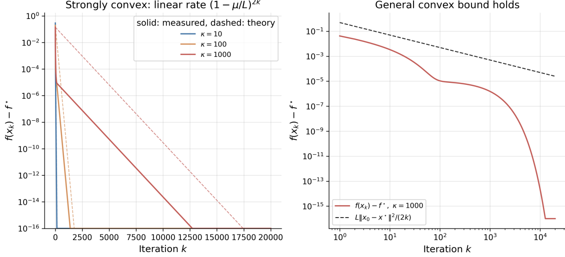
Figure 57: Left: optimality gap f(x_k) - f^* of gradient descent with step 1/L on strongly convex quadratics at condition numbers \kappa \in \{10, 100, 1000\} (solid), against the geometric envelope (1 - \mu/L)^{2k} (dashed), on a log scale. Right: the worst-conditioned case ( \kappa = 1000 ) against the general convex bound L\|x_0 - x^*\|^2/(2k) (dashed), on log-log axes, which it stays below throughout.
