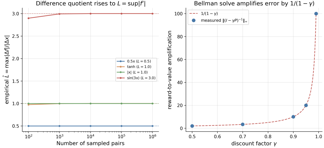
Figure 61: Left: the empirical Lipschitz constant \hat{L} , the largest difference quotient |f(x) - f(y)|/|x - y| over sampled pairs, approaching the analytic L = \sup|f'| (dashed) from below for four scalar functions, on a log-scaled pair count; the two piecewise-linear cases ( 0.5x , |x| ) sit at L already at the smallest sample size. Right: the reward-to-value amplification \|(I - \gamma P)^{-1}\|_\infty of the policy-evaluation solve against the discount factor \gamma (markers), matching 1/(1 - \gamma) (dashed).
