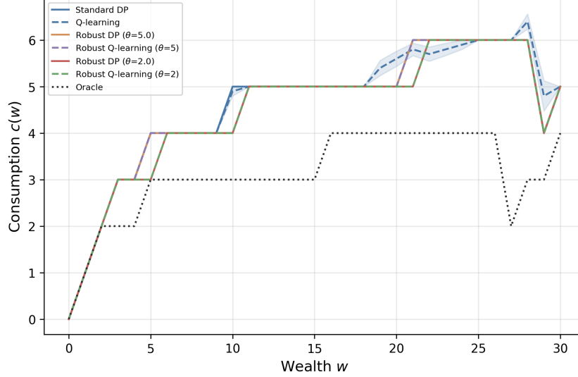
Figure 43: Consumption policy c(w) for each method. Dashed lines show Q-learning policies; solid lines show DP.
