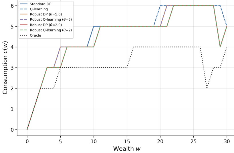
Figure 28: Consumption policy c(w) for each method. Dashed lines show Q-learning policies; solid lines show DP.
