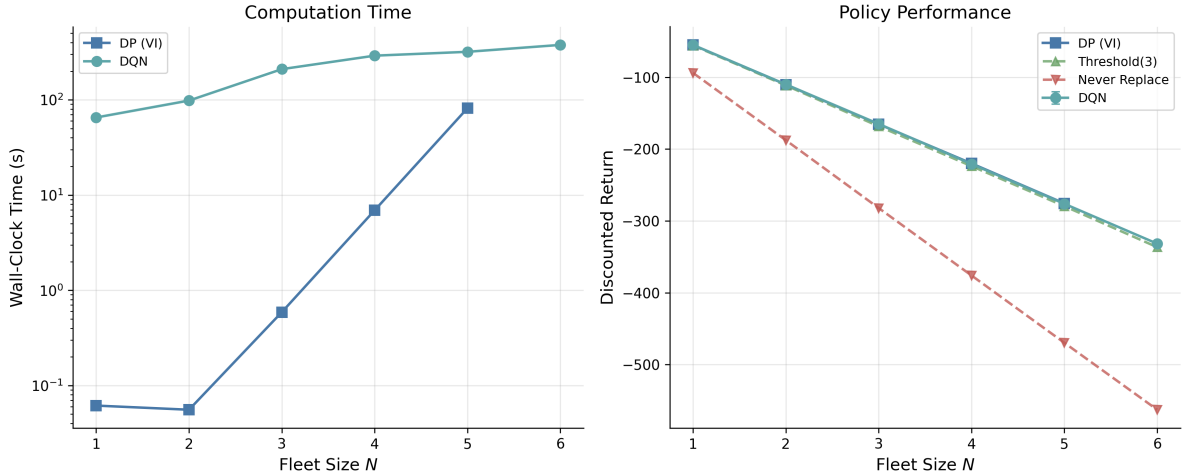
Figure 12: Bus engine replacement benchmark. Left: computation time vs. fleet size (log scale). Right: discounted return vs. fleet size for DP, DQN, and heuristic baselines. At N = 6 (46,656 states), DP is infeasible (no data point).
