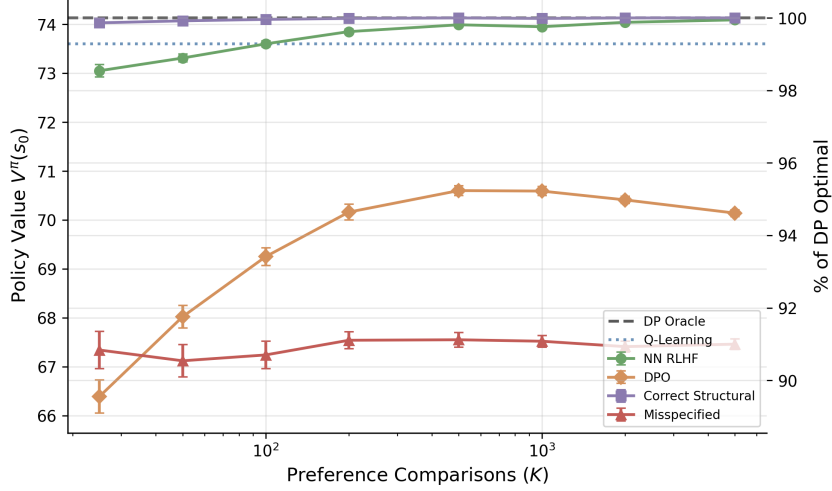
Figure 22: Policy value V^\pi(s_0) versus number of preference comparisons K for all six methods (30 seeds, L = 15 ). The right axis shows the percentage of DP-optimal value.
