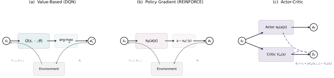
Figure 1: Architecture comparison of three core algorithm families: value-based, policy gradient, and actor-critic. (a) DQN maps states to Q-values for all actions, selecting the argmax. (b) REINFORCE maps states to a probability distribution over actions, then samples. (c) Actor-Critic maintains separate policy and value networks. Panels (a) and (b) depict the acting-time forward pass; panel (c) additionally shows the critic’s TD error \delta_t feeding back to both networks during training, which yields lower-variance policy updates than REINFORCE’s Monte-Carlo return.
