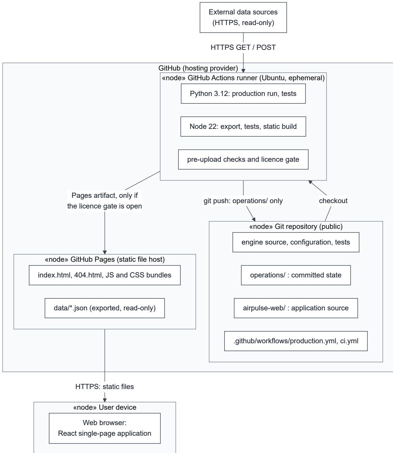
Figure 6. Deployment diagram.
