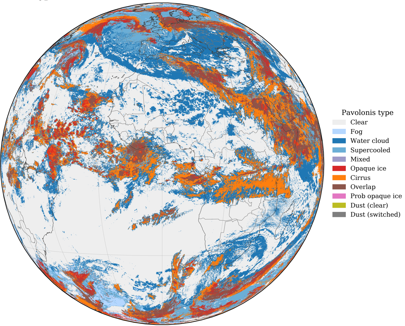
Cloud type — R11 2026-02-25 13:12 UTC
