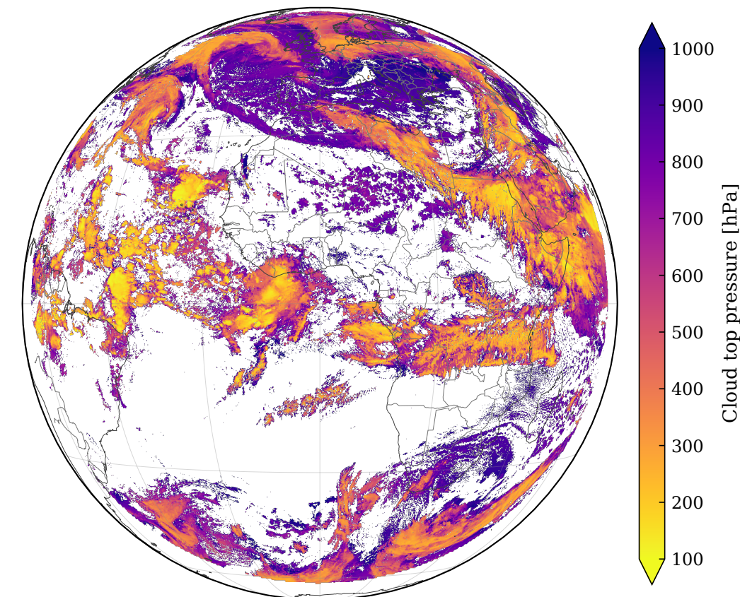
CTP — R11 2026-02-25 13:12 UTC
