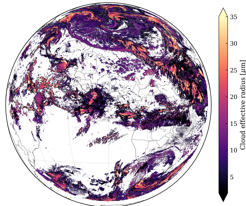
CER — R11 2026-02-25 13:12 UTC
