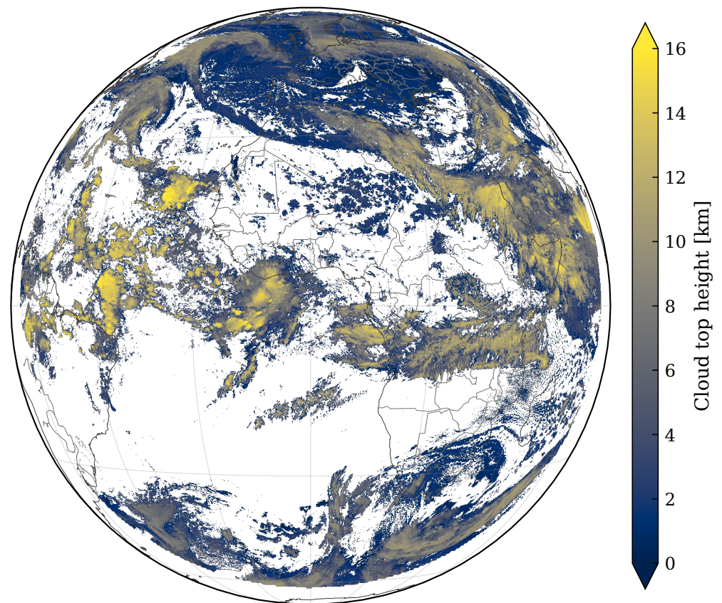
CTH — R11 2026-02-25 13:12 UTC
