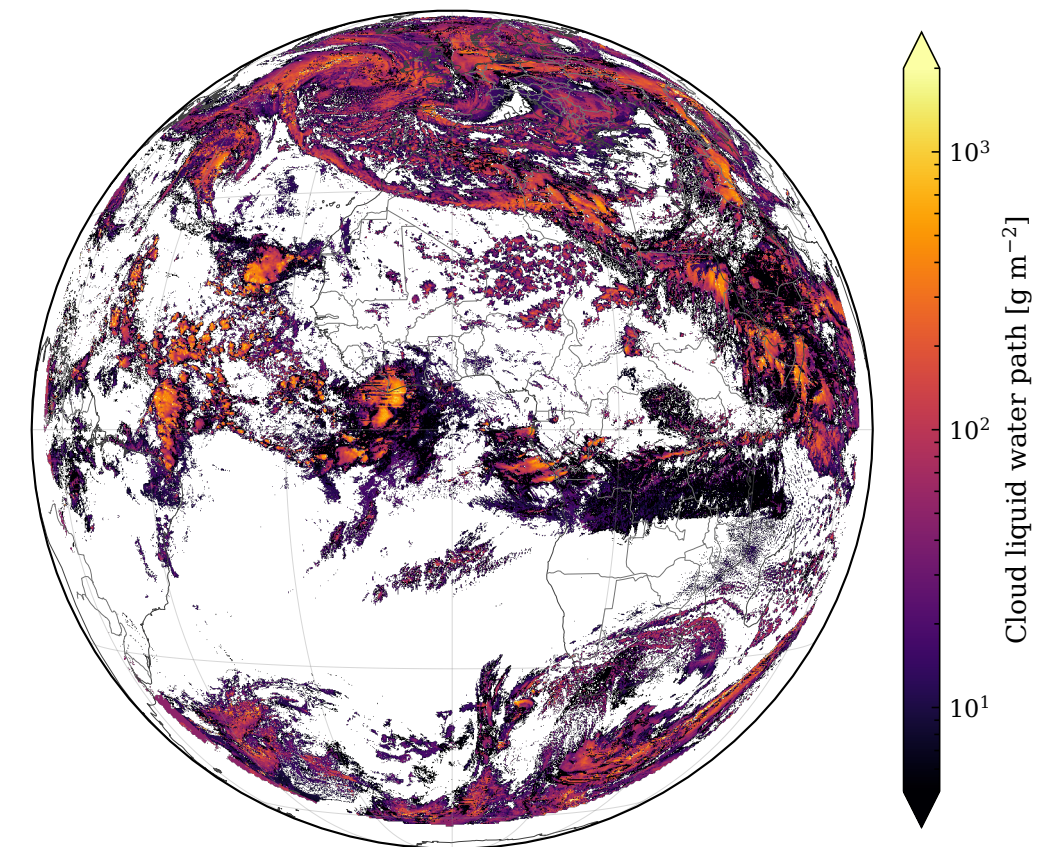
CWP — R11 2026-02-25 13:12 UTC
