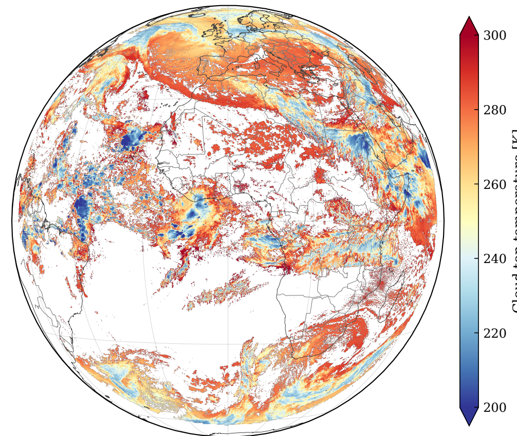
CTT — R11 2026-02-25 13:12 UTC
