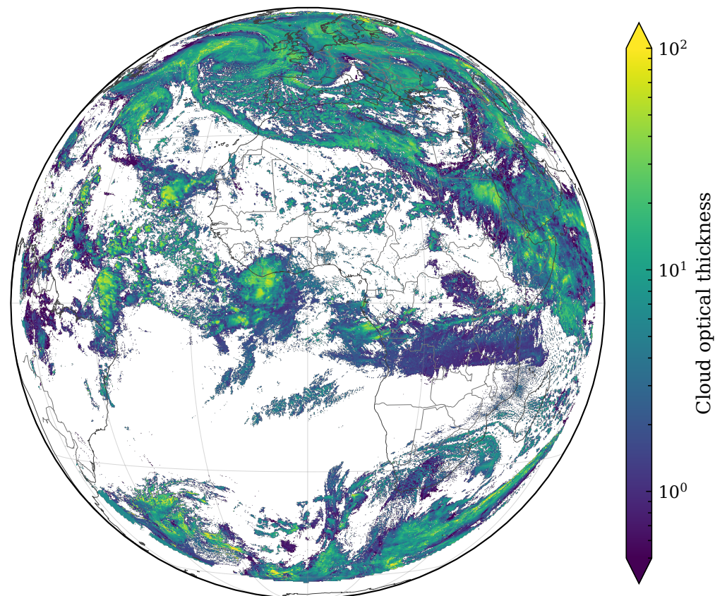
COT — R11 2026-02-25 13:12 UTC
