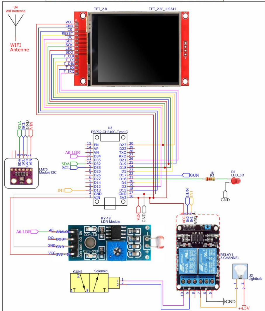
Reciever - Ground Control Station
