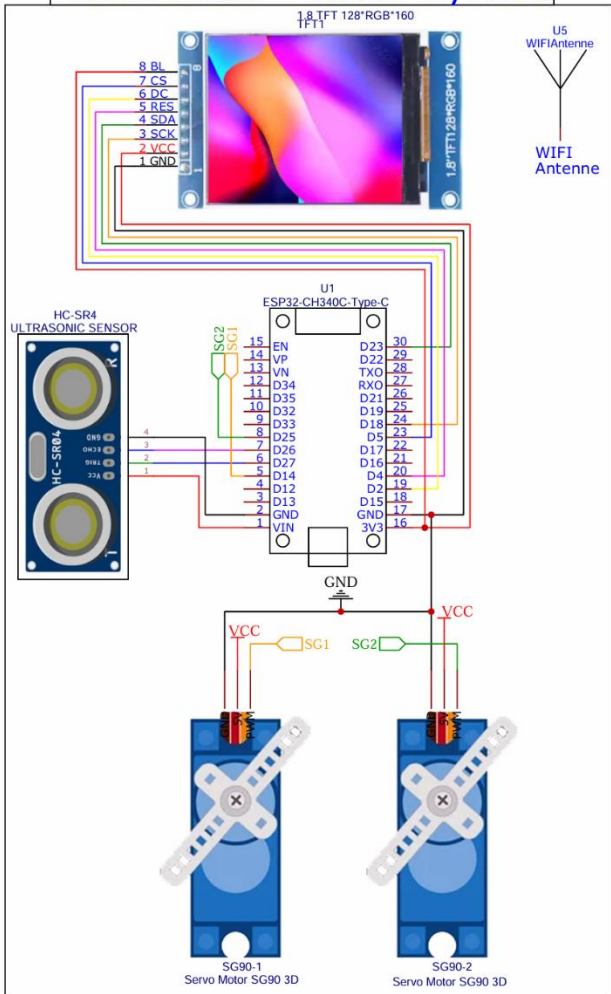
Transmitter - Radar System
