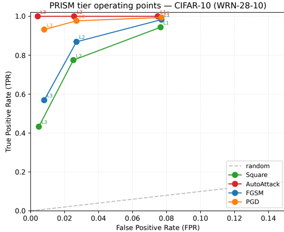
(a) CIFAR-10 (WRN-28-10).
