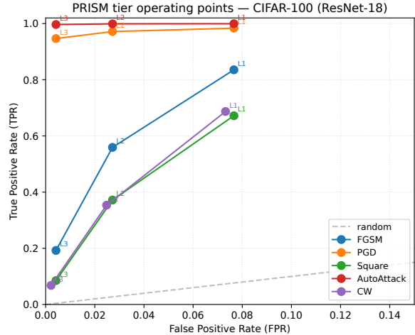
(b) CIFAR-100 (ResNet-18).
