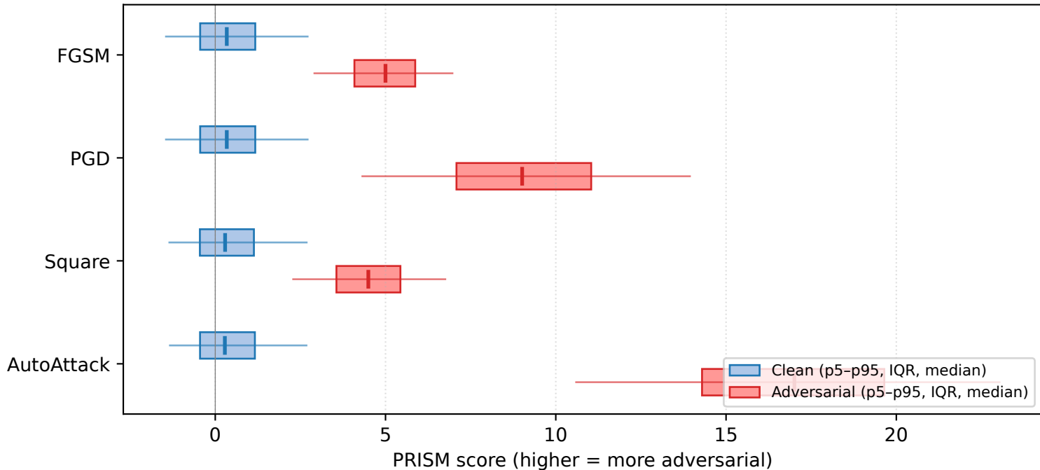
Score distributions: clean (blue) vs adversarial (red) — CIFAR-10 (WRN-28-10)
