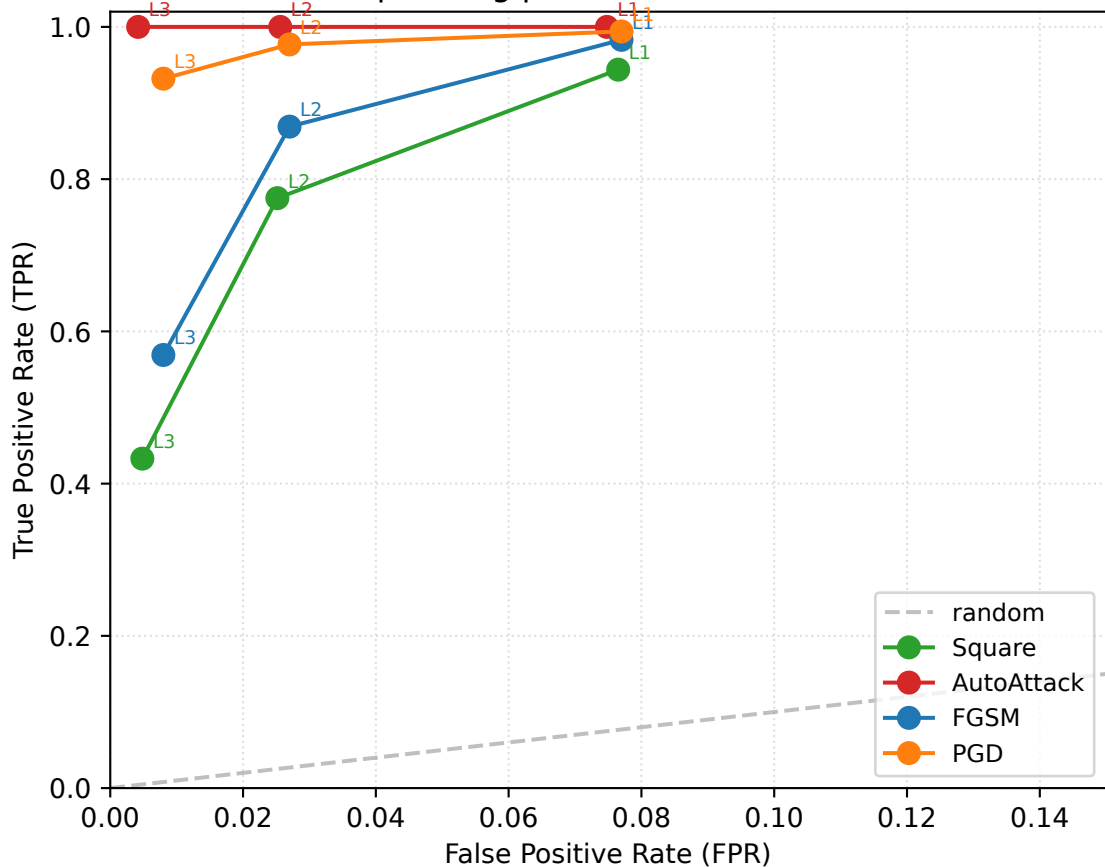
PRISM tier operating points — CIFAR-10 (WRN-28-10)
