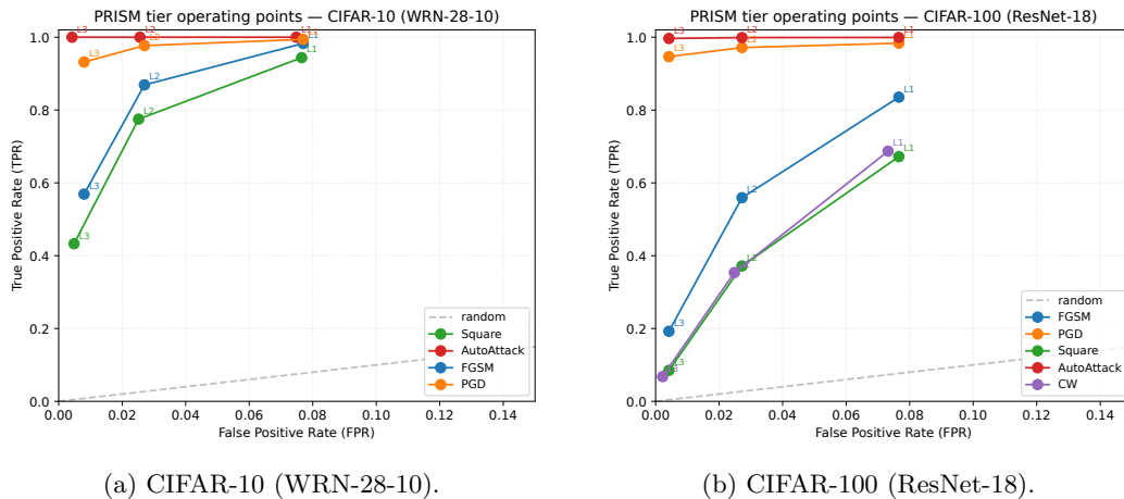
Figure 3: PRISM three-tier operating points (L1, L2, L3) per attack. AutoAttack and PGD saturate near TPR=1 even at the tight L3 FPR ( \leq 0.005 ); Square trades TPR for tighter FPR most steeply, consistent with its score-based attack signature being the weakest of the four in the ensemble feature space.
