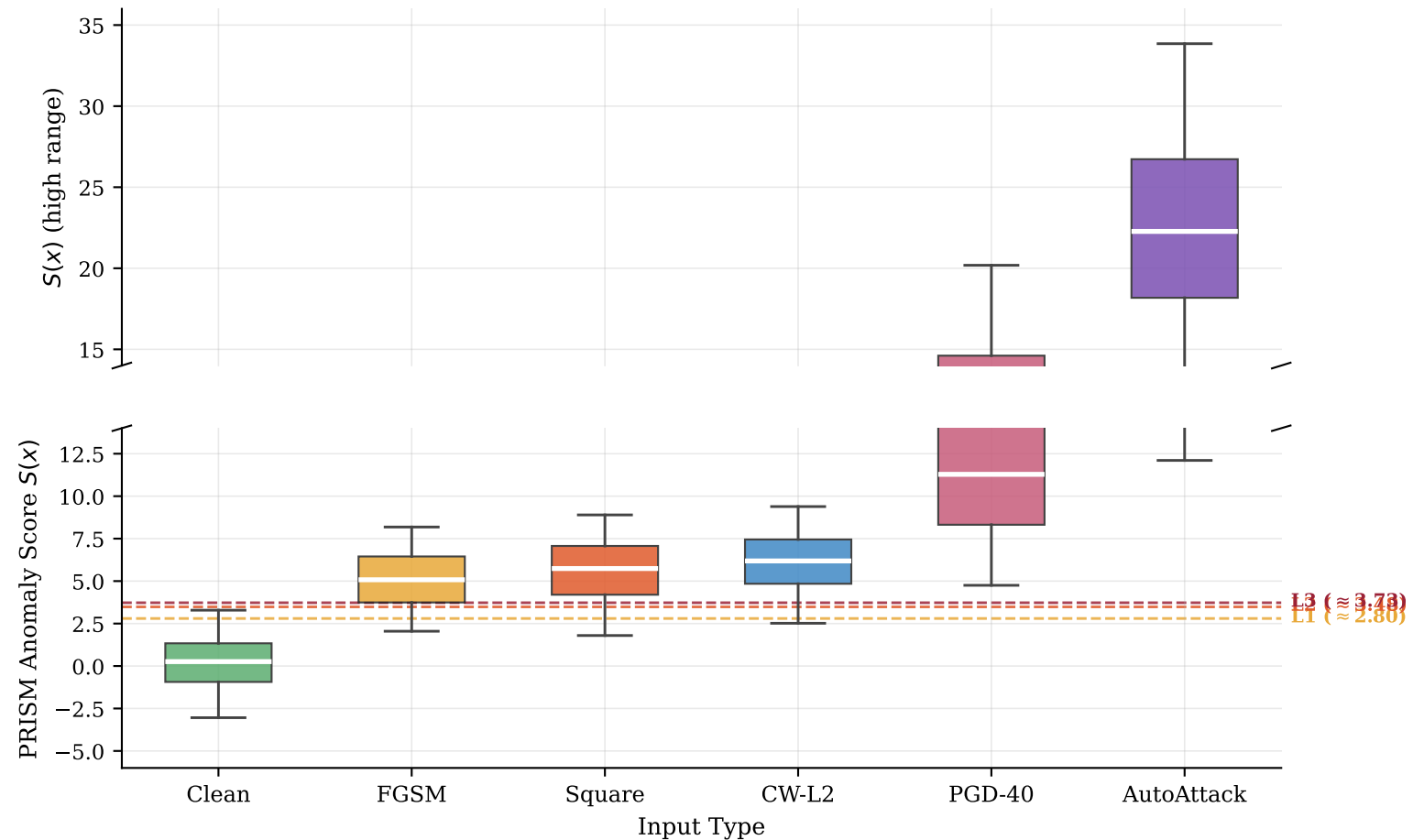
Canonical Ensemble Score Distribution — Clean vs Adversarial (5-seed pooled quantiles: whiskers = p05/p95, box = IQR, line = median)
