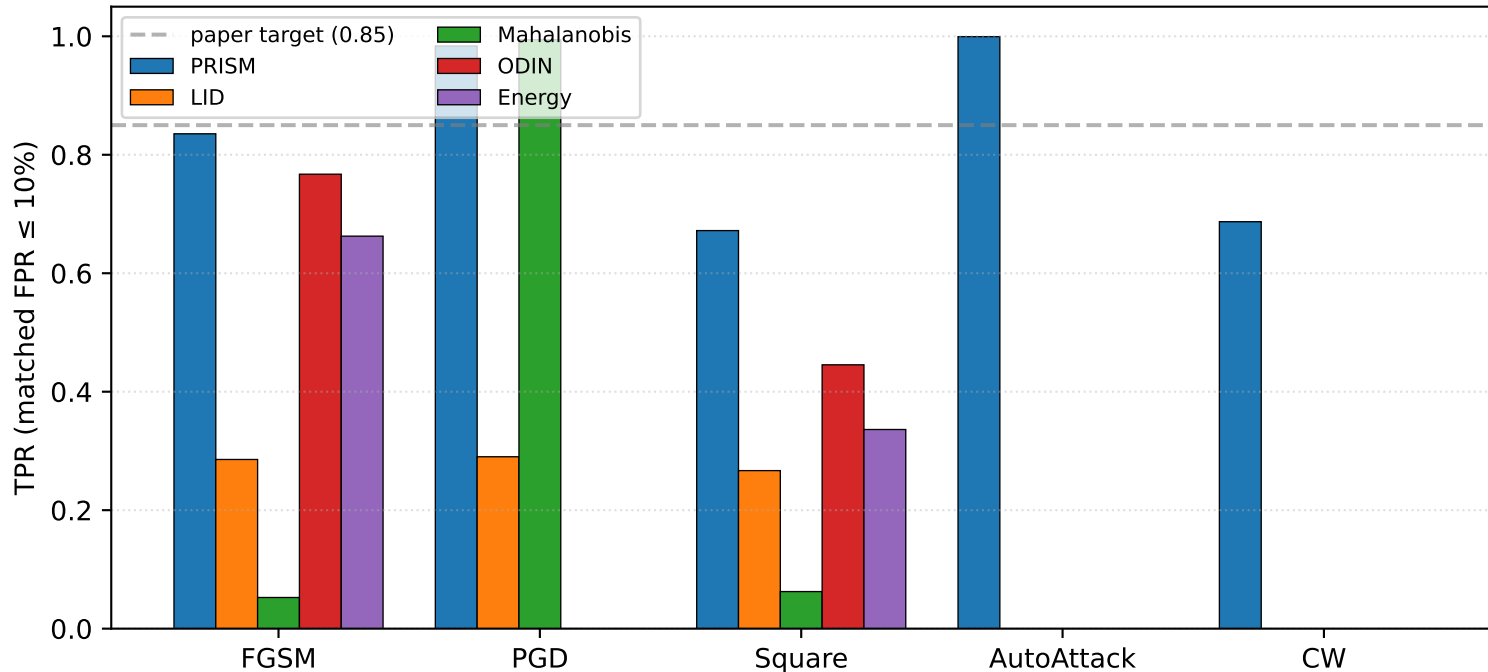
PRISM vs baselines — CIFAR-100 (ResNet-18)
