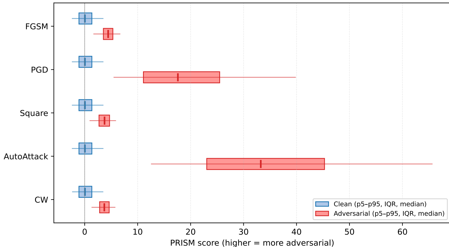
Score distributions: clean (blue) vs adversarial (red) — CIFAR-100 (ResNet-18)
