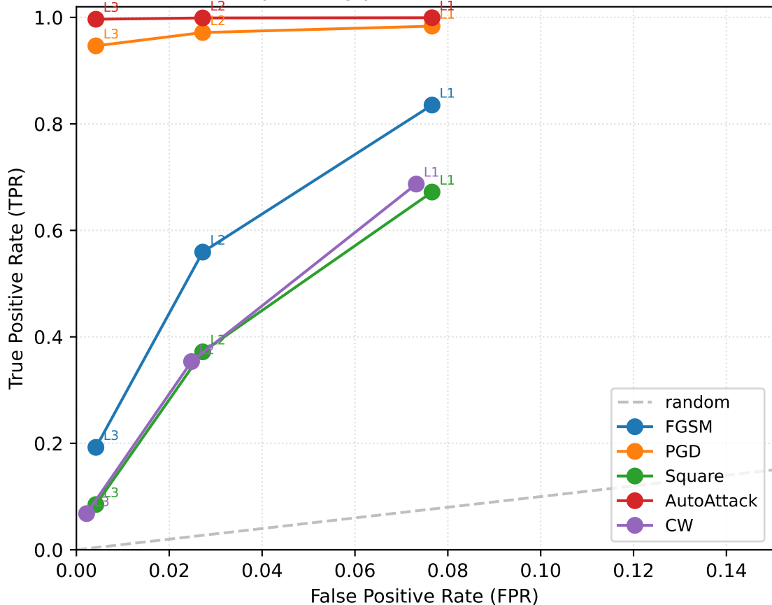
PRISM tier operating points — CIFAR-100 (ResNet-18)
