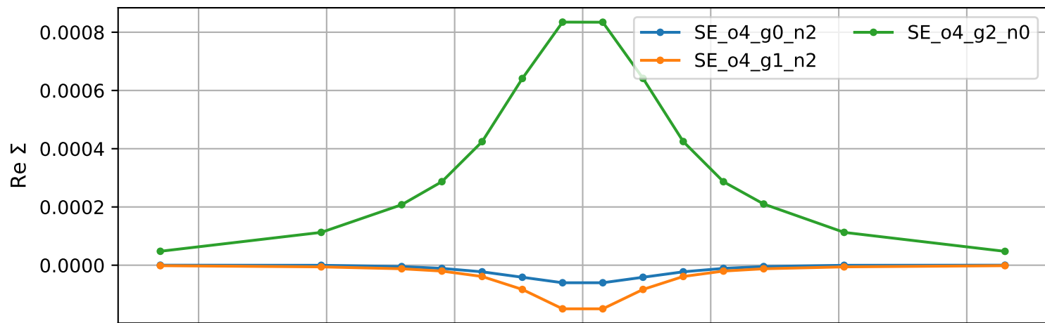
Three fourth order diagram considered k = [\pi, \pi]
