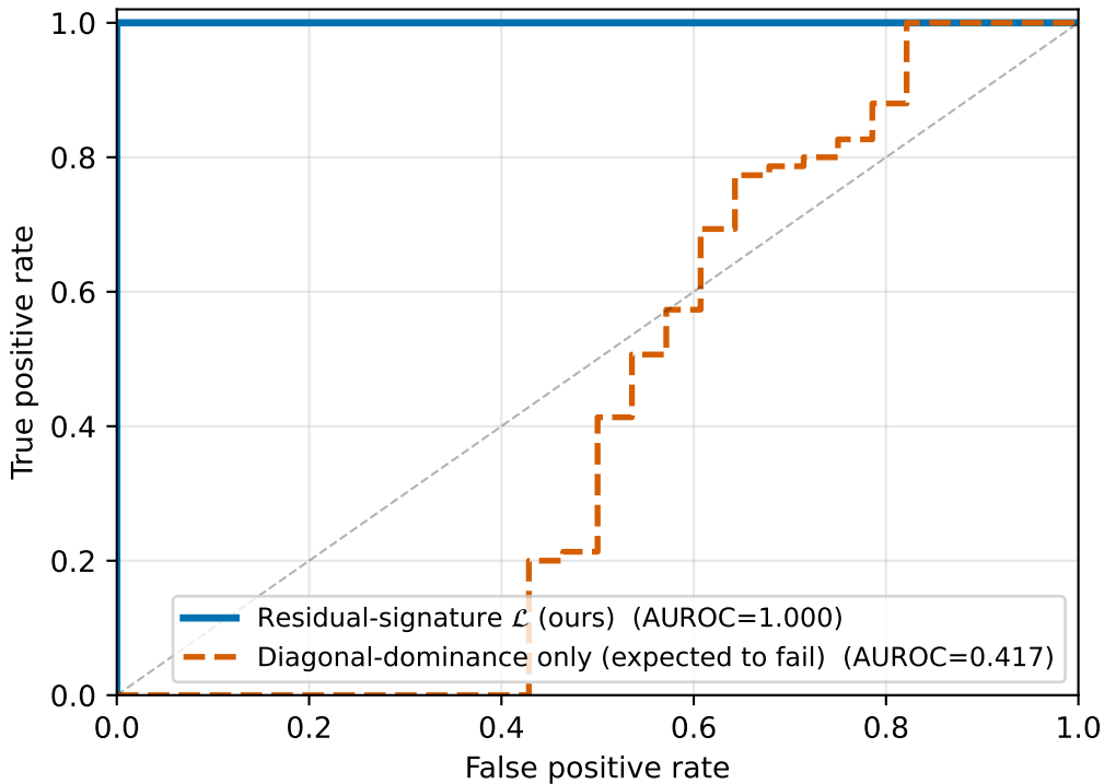
(b) ROC: lineage detection
