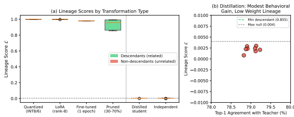
Figure 6: GPT-2-Small-Lite lineage benchmark (8 roots, 120 pairs across all splits; Table 7 reports results on the 3 held-out test roots, 45 pairs). (a) Lineage scores by transformation type. Descendants (green) score high; non-descendants (red) score near zero. (b) Distillation modestly improves teacher–student agreement (79% top-1, +1.4 points over independent training) while leaving the weight-lineage score near the independent-root range, confirming that behavioral similarity \neq weight inheritance.
