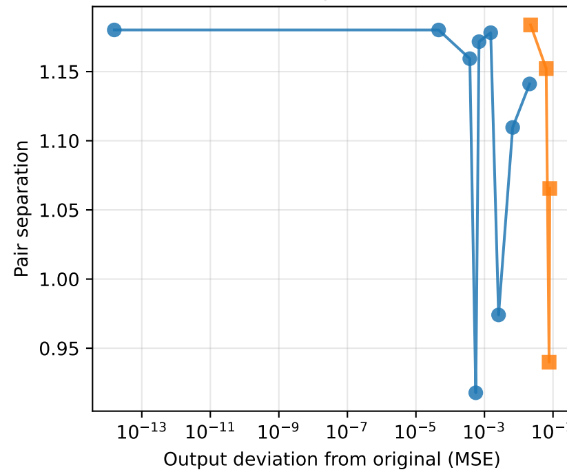
Pair separation
