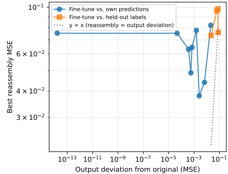
Reassembly tracks attack-induced drift
