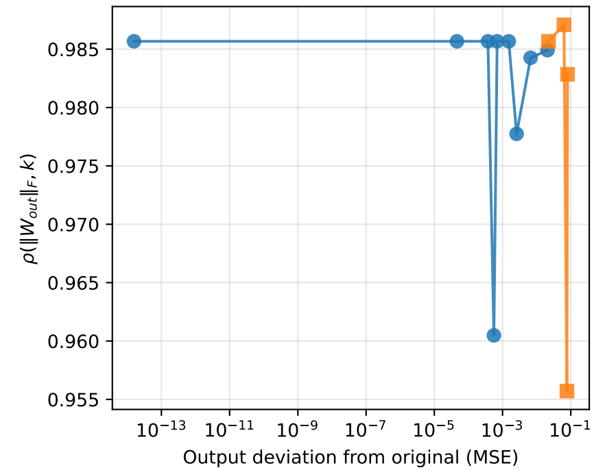
\rho(\|W_{out}\|_F, k)
