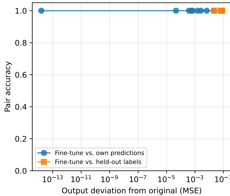
Pair accuracy
