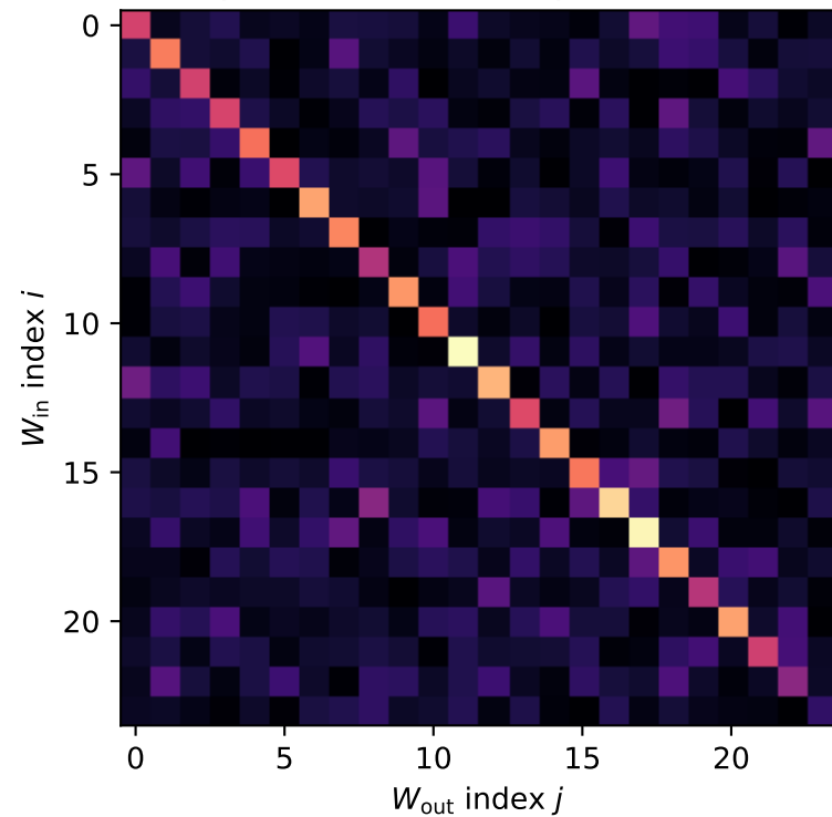
(a) ResNet (trained) pair acc = 1.00, sep = +0.01
