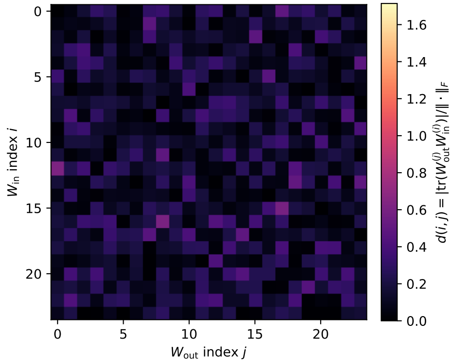
(b) PlainNet (trained, no skip) pair acc = 0.00, sep = -0.56
