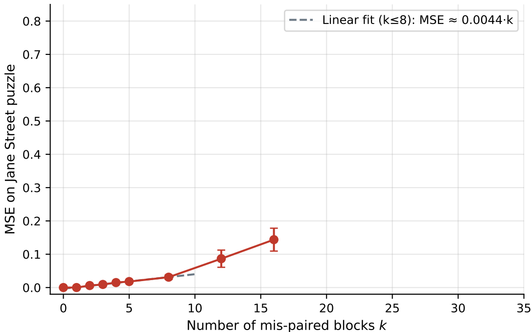
The Pairing Wall: MSE vs. k mis-paired blocks (ordering held at ground truth)
