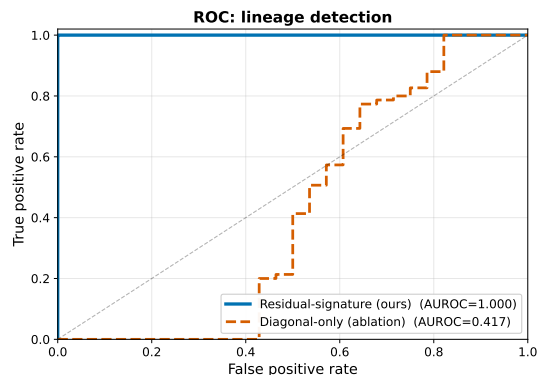
Figure 6: ROC for lineage verification on depth-24 residual MLPs. The residual-signature score achieves AUROC=1.000; diagonal-dominance alone fails (AUROC=0.417) because it cannot distinguish two trained residual models.
