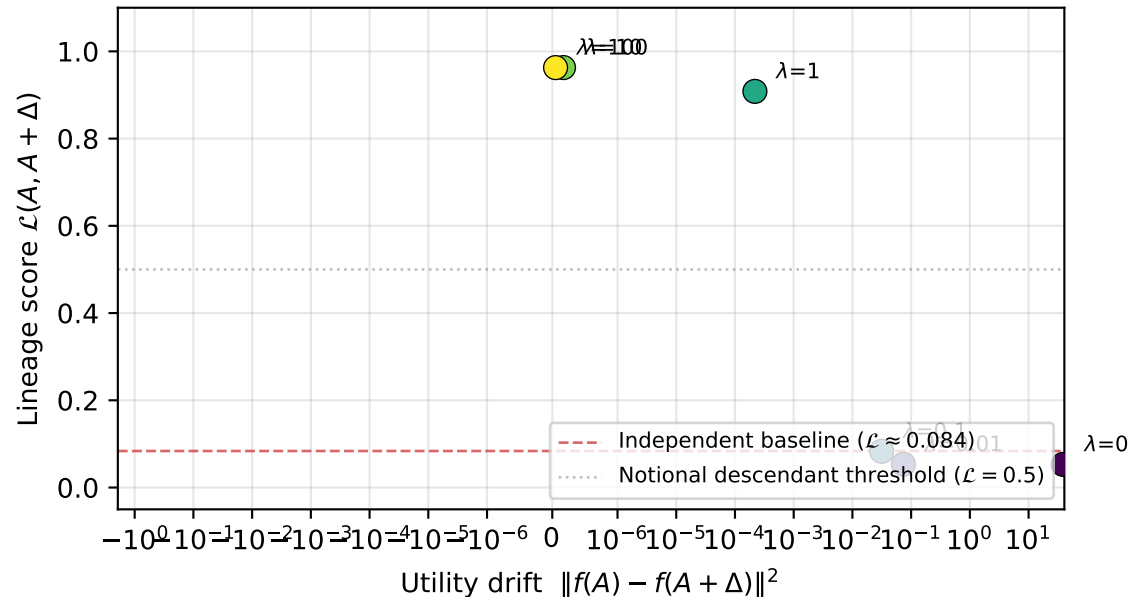
(b) Gradient-attack Pareto curve
