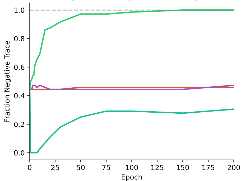
Negative Trace (Dynamical Isometry)
