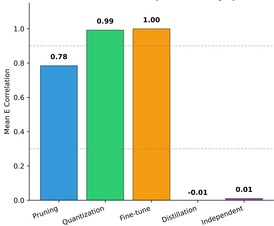
Mean E Correlation by Method Category
