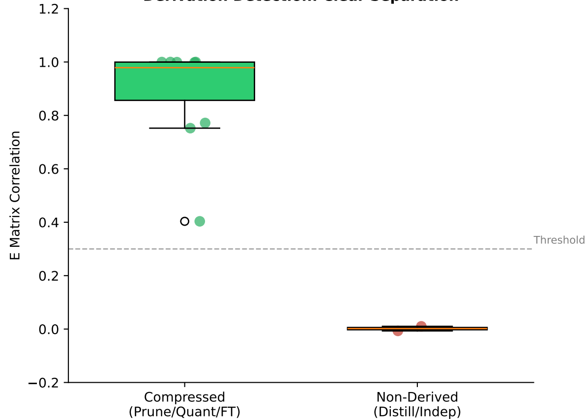
Derivation Detection: Clear Separation
