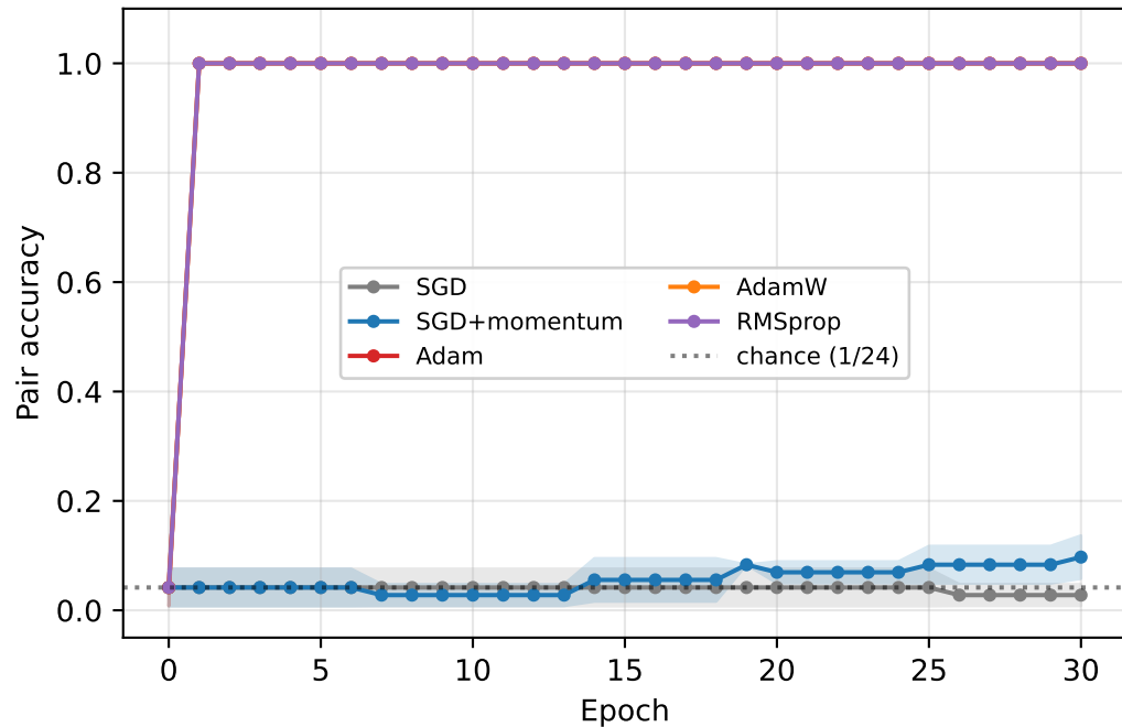
A. Fingerprint emerges only under adaptive optimizers
