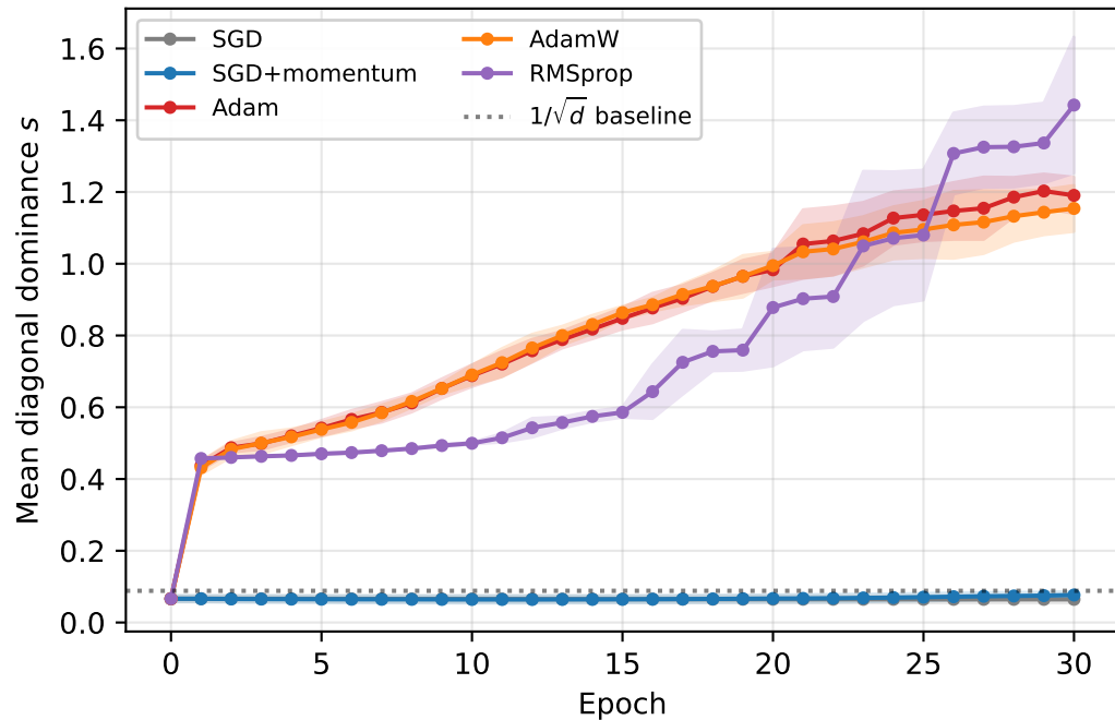
B. Diagonal structure climbs only with Adam/AdamW/RMSprop
