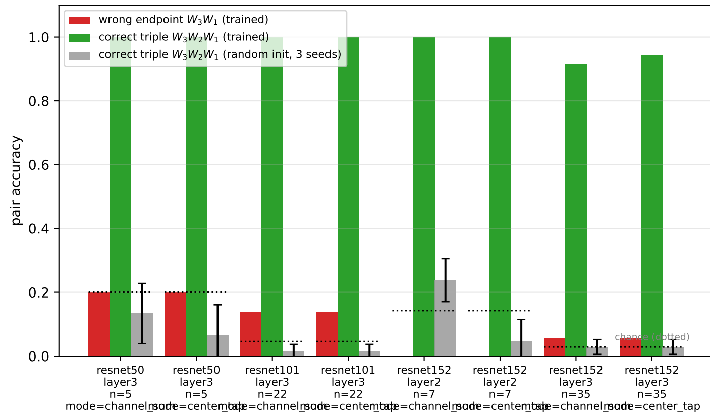
(a) Wrong vs correct factorization on Bottleneck ResNets
