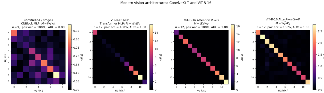
Figure 15. Diagonal-dominance matrices on modern vision architectures. (a) ConvNeXt-T stage 3 (9 CNBlocks) pairs at 100% via the MLP product W_2W_1 . (b) ViT-B/16 MLP (12 blocks) also pairs at 100% with AUC 1.000 and a strong depth-coded brightness gradient. (c) ViT-B/16 attention V \leftrightarrow O produces the single cleanest pair signal in this paper: \text{sep} = +4.84 , \text{AUC} = 1.000 , and 100% of correctly-paired products have negative trace — the full Proposition 1 prediction. (d) ViT-B/16 attention Q \leftrightarrow K also recovers 100% on a smaller absolute scale.
