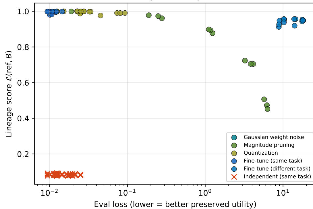
(c) Lineage vs utility tradeoff
