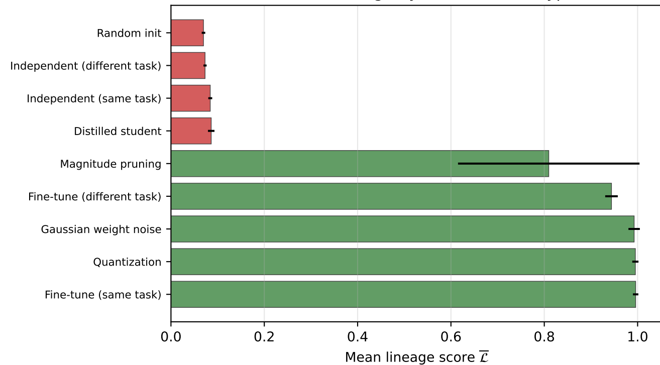
(d) Mean lineage by attack/control type
