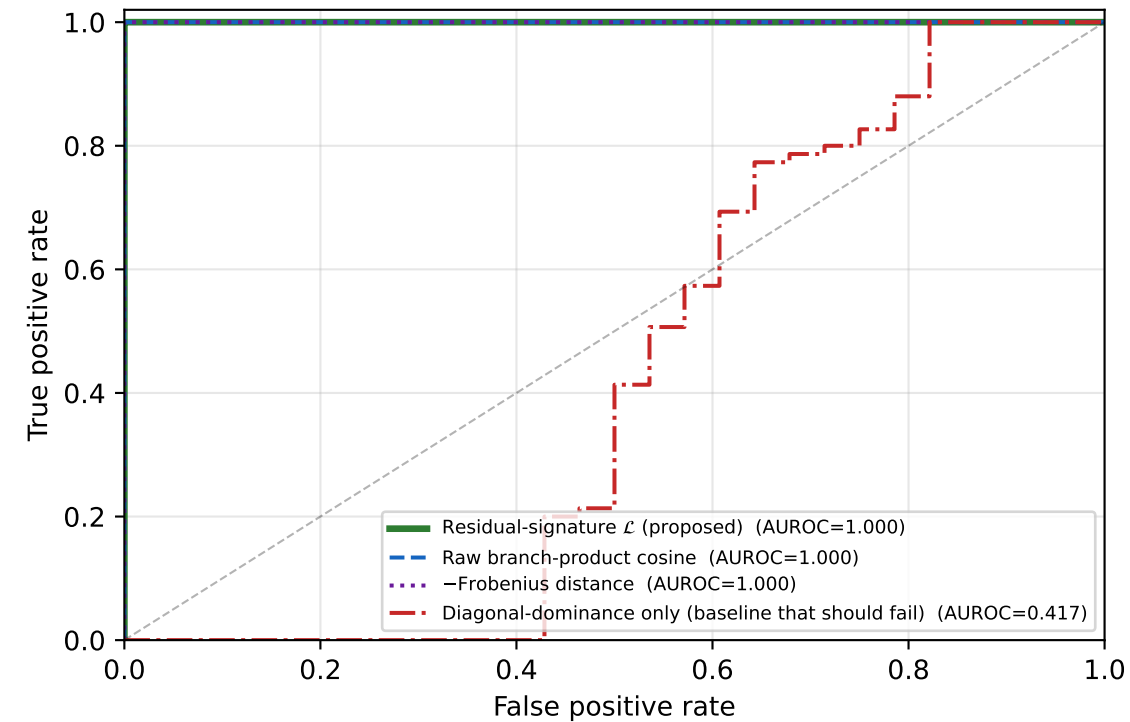
(b) ROC: descendant vs non-descendant
