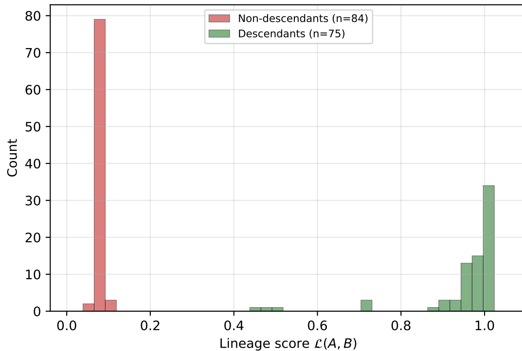
(a) Score distributions
