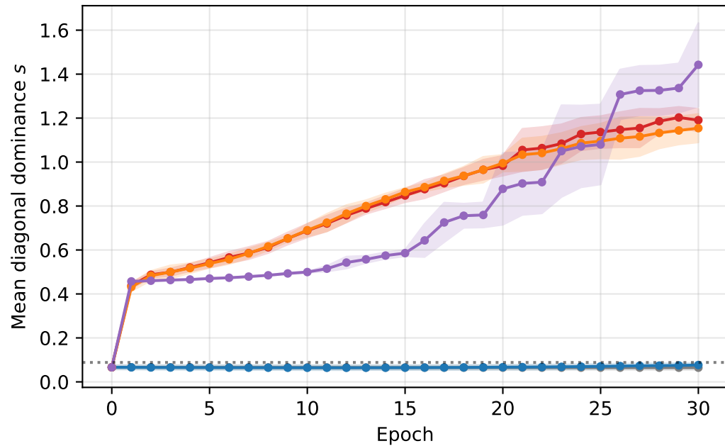
B. Diagonal structure climbs only with Adam/AdamW/RMSprop
