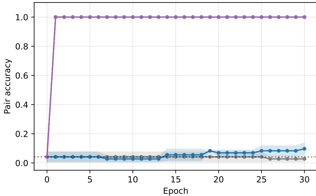
A. Fingerprint emerges only under adaptive optimizers
