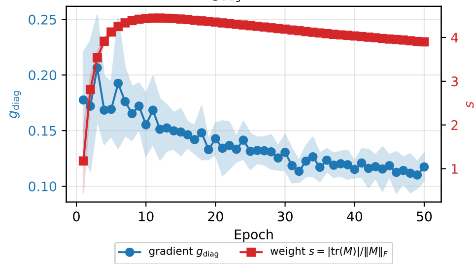
A. Gradients stay flat while weights climb Pearson r(g_{\text{diag}}, s) = -0.12 \pm 0.09
