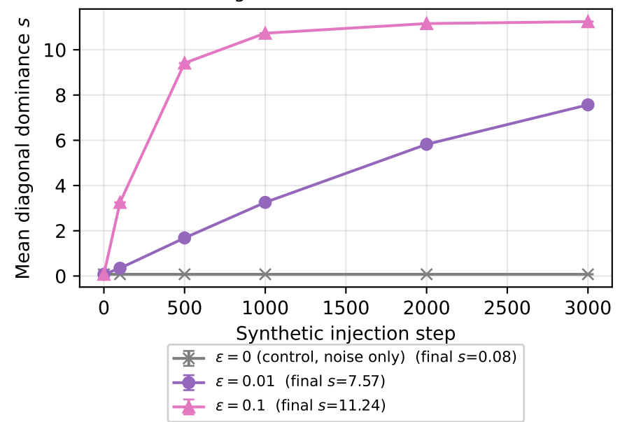
C. Diagonal injection (no backprop) builds the fingerprint Diagonal structure is sufficient
